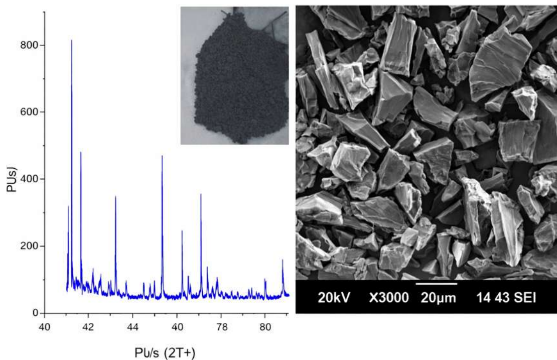
Fig. 1. SEM micrograph and XRD spectra of 'as received' SiC powder
