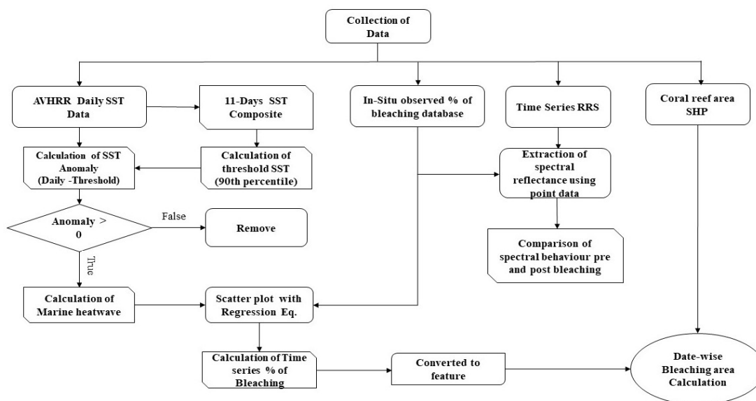
Figure 2: Flow chart of the MHW computation: (i) daily NOAA AVHRR SST anomaly computed relative to the 90th-percentile climatology; (ii) contiguous positive anomalies merged if the gap is \leq 2 days; (iii) cumulative weighted sum converted to MHW(%)
