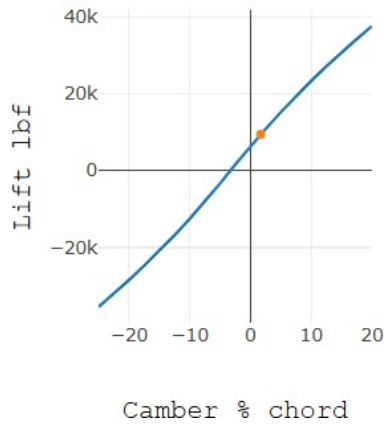
Lift Vs Camber
