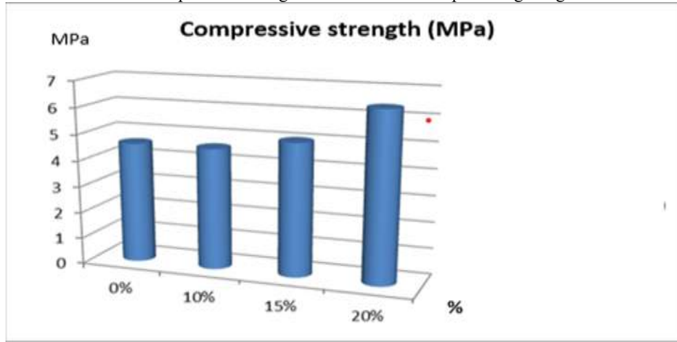
Figure 9: Variation in compressive strength as a function of glass content
