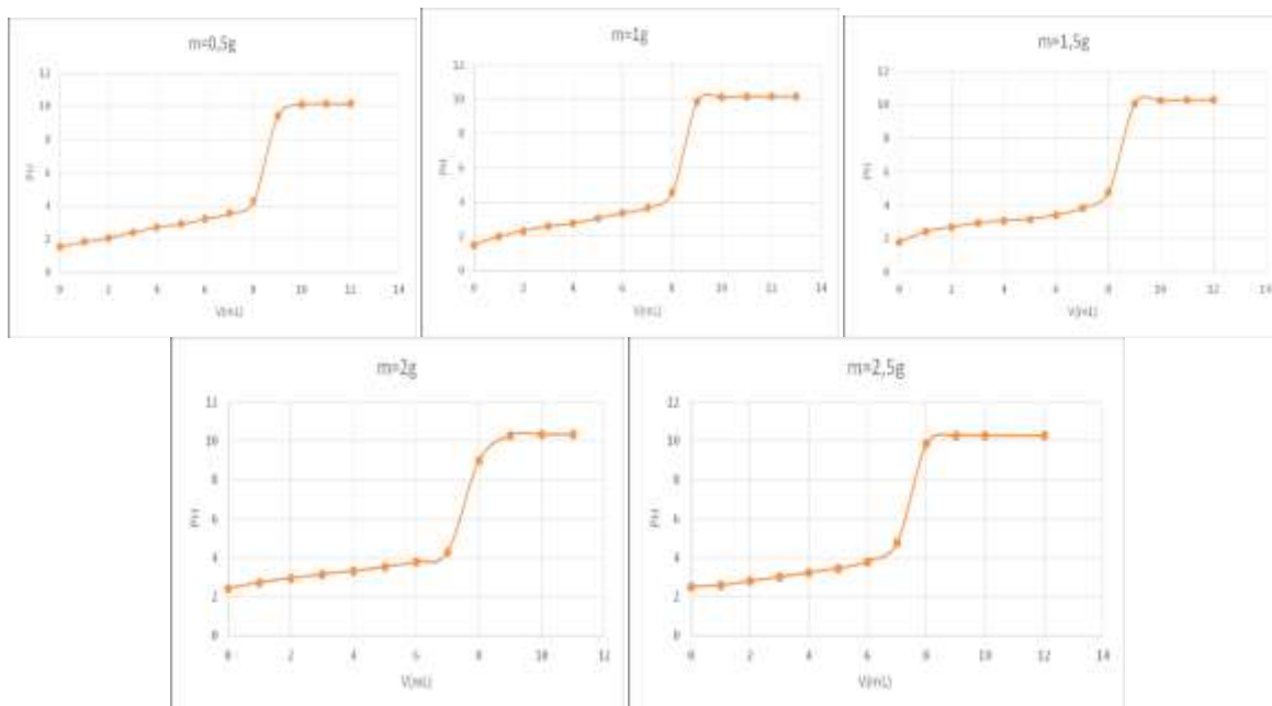
Fig.11: Analysis of the filtrate (10 cm 3 ) after treatment with acetic acid (0.196 N) of Youssoufia phosphate ore processed in a muffle furnace at 85°C (m = 0.5 g, m = 1 g, m = 1.5 g, m = 2 g, and m = 2.5 g)
