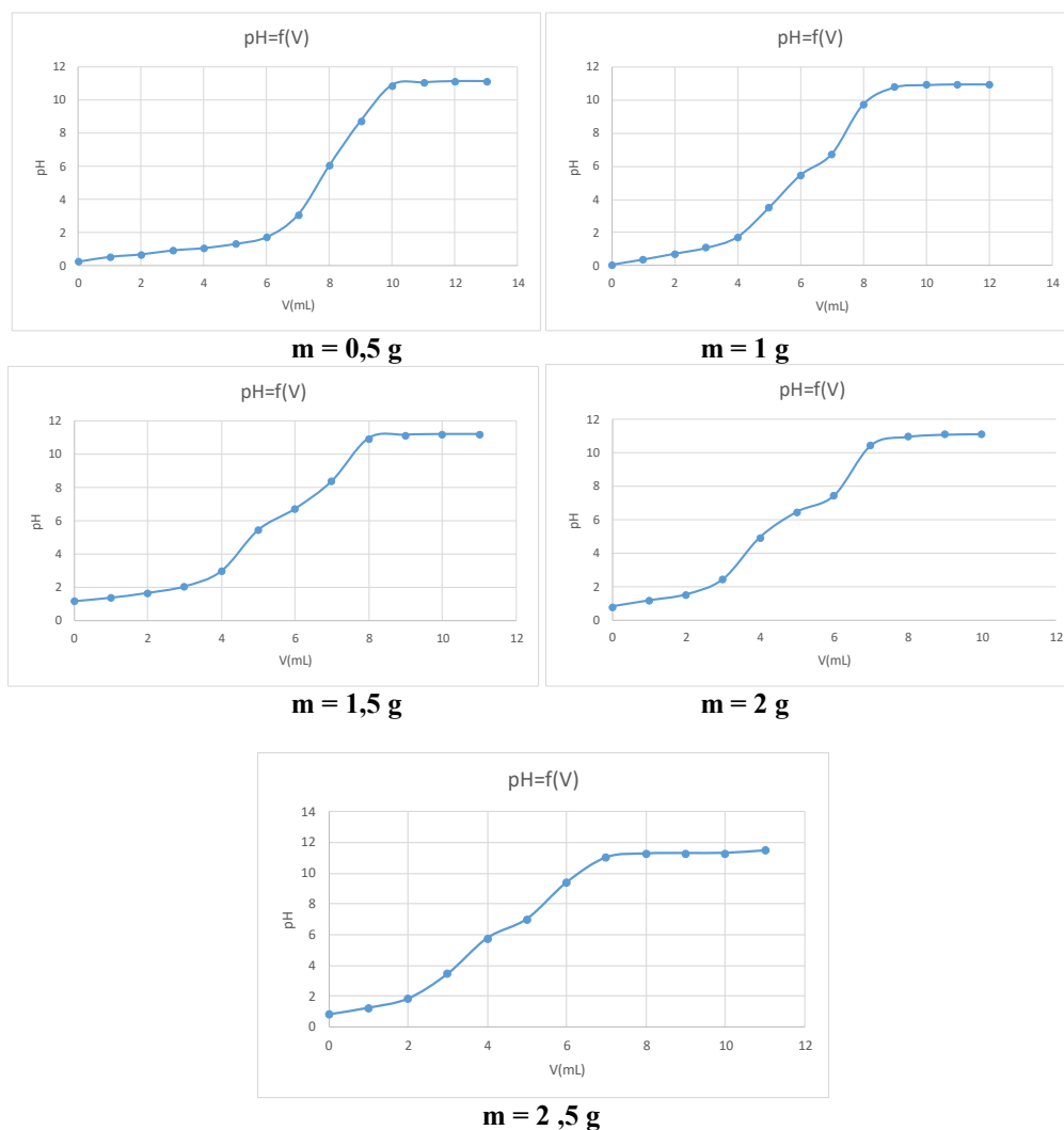
Fig: 8 Analysis of the filtrate (10 cm 3 ) after treatment with sulfuric acid (0.195 N) of Youssoufia phosphate ore processed in a muffle furnace at 550°C (m = 0.5 g, m = 1 g, m = 1.5 g, m = 2 g, and m = 2.5 g)
