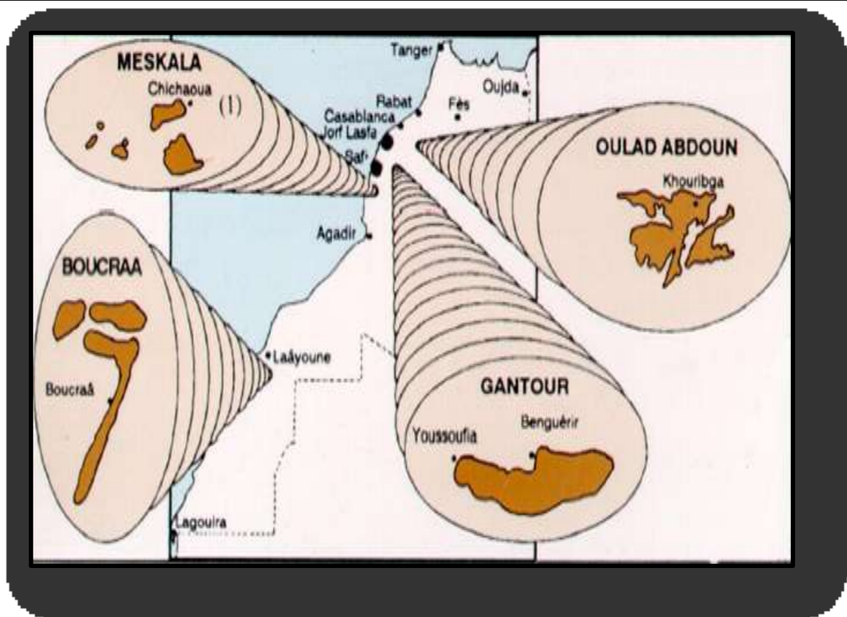
Fig.1: The four phosphate deposits in Morocco
