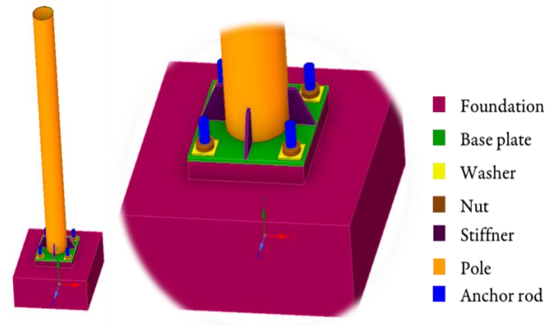
Figure 3: Realistic modeling of the candelabra
