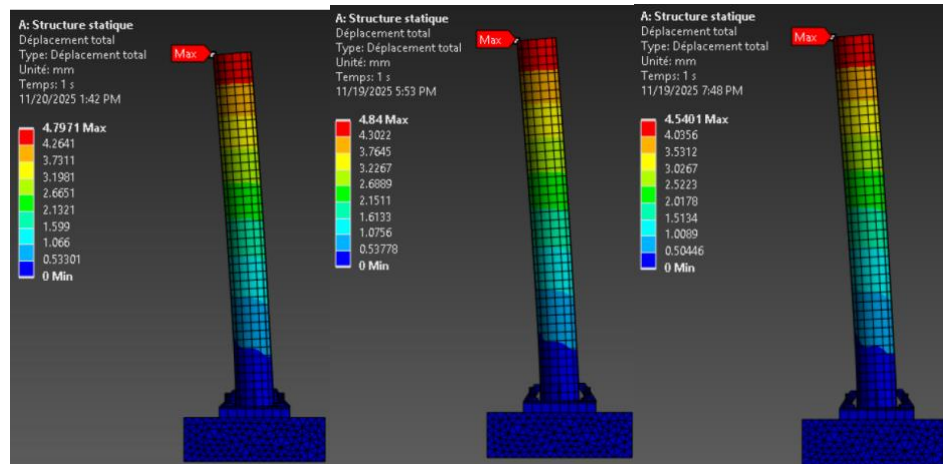
Case 1 Case 2 Case 3 Figure 20: Displacement mapping of different stiffener models analyzed
