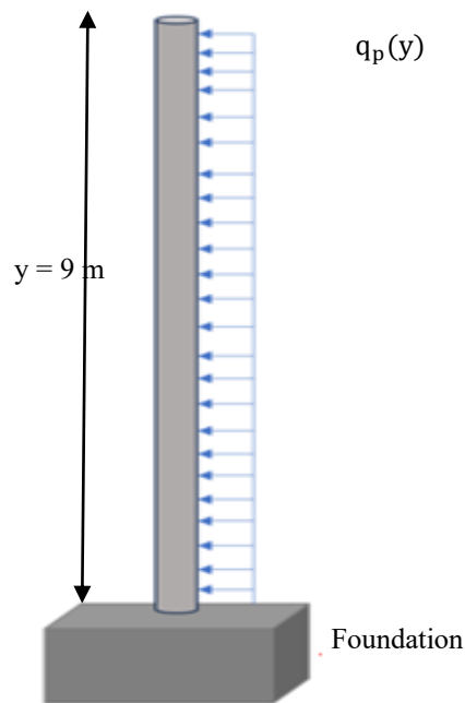
Figure 8: Illustration of the wind pressure on the candelabra
