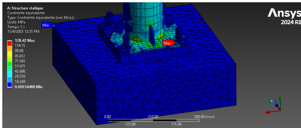
Case 1: 4 anchor rods
