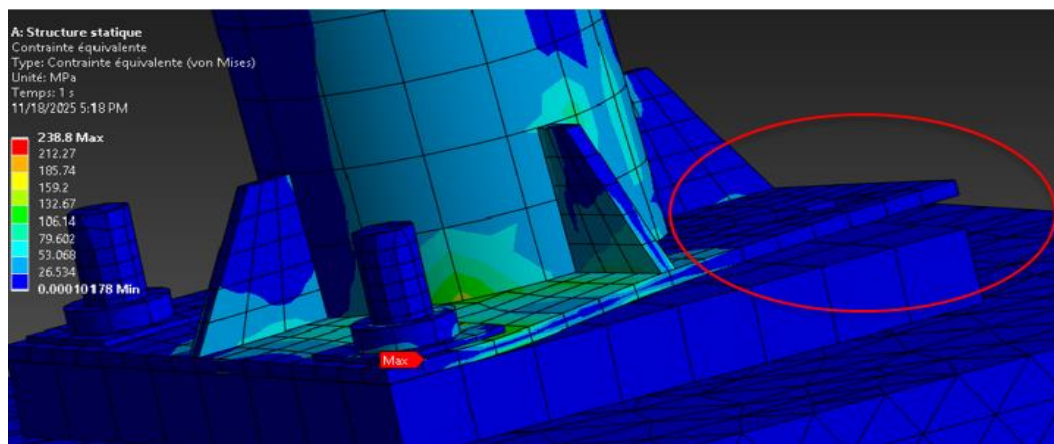
Figure 17: Plate detachment in case 2
