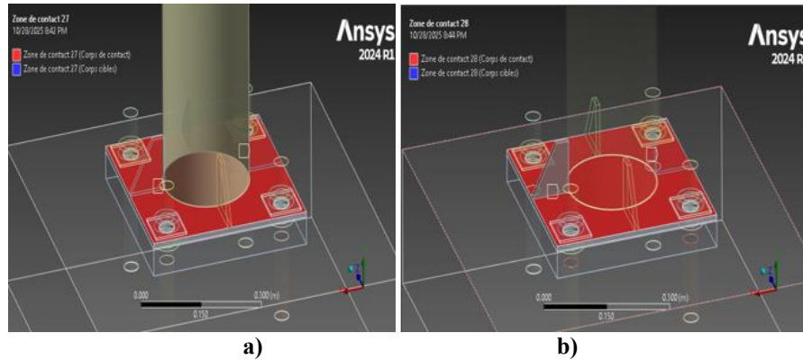
Figure 7: a) Contact between plate and pole; b) Contact between stiffener and plate
