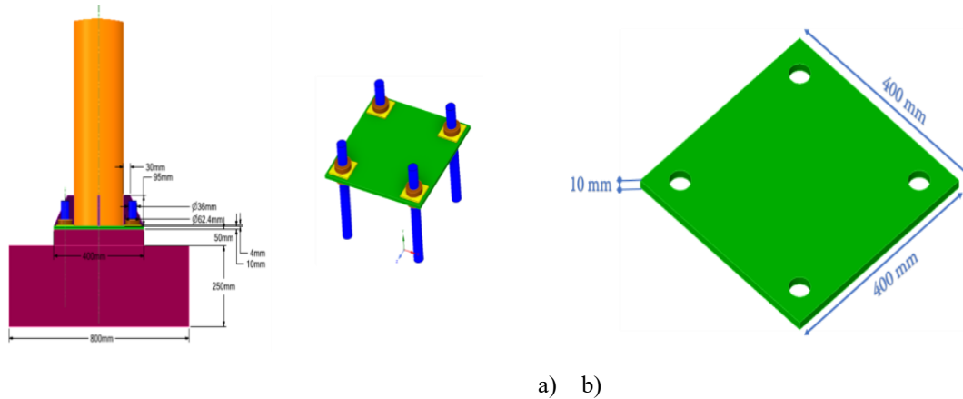
Figure 4: a) Dimensions of the pole base, front view of the model, b) Base plate dimensions
