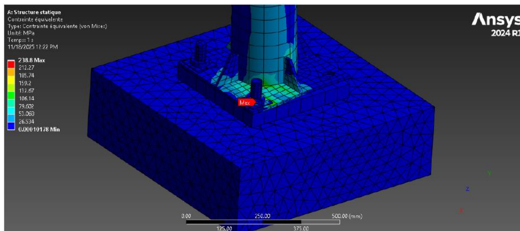
Case 2: 3 anchor rods
