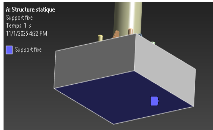
Figure 10: Boundary Condition
