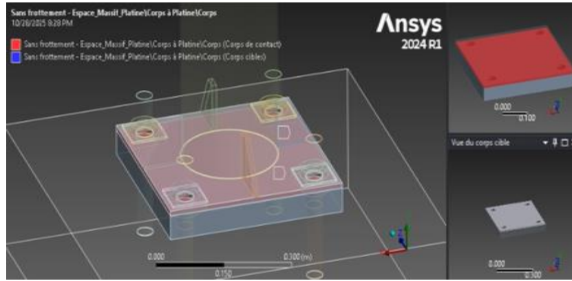
Figure 6: Frictionless contact between the plate and the concrete mass
