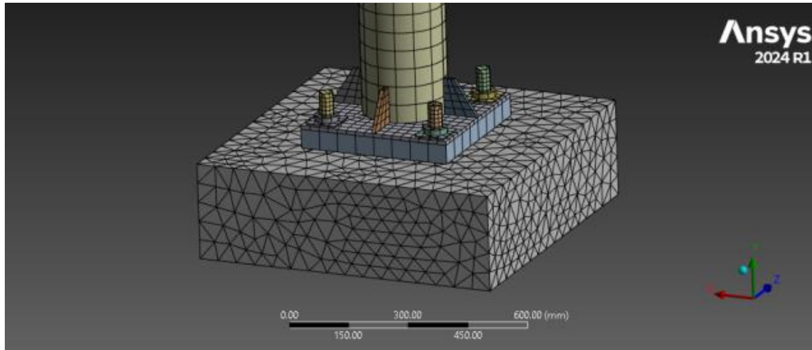
Figure 11: Mesh of finite element model
