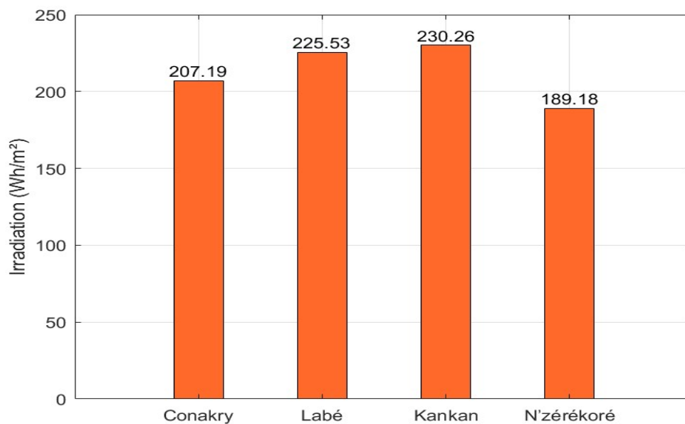
Figure 3: Time-series trends in solar radiation for the regions, annual average
