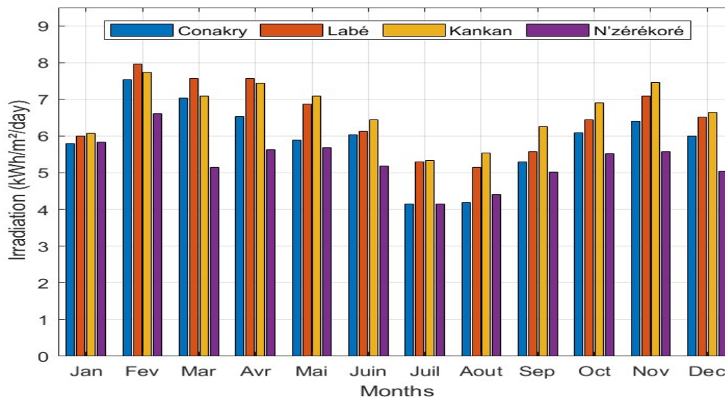
Figure 5: Trends in Monthly Average Daily Irradiation by Region
