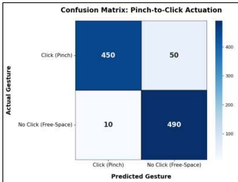
Figure.2. Confusion Matrix
