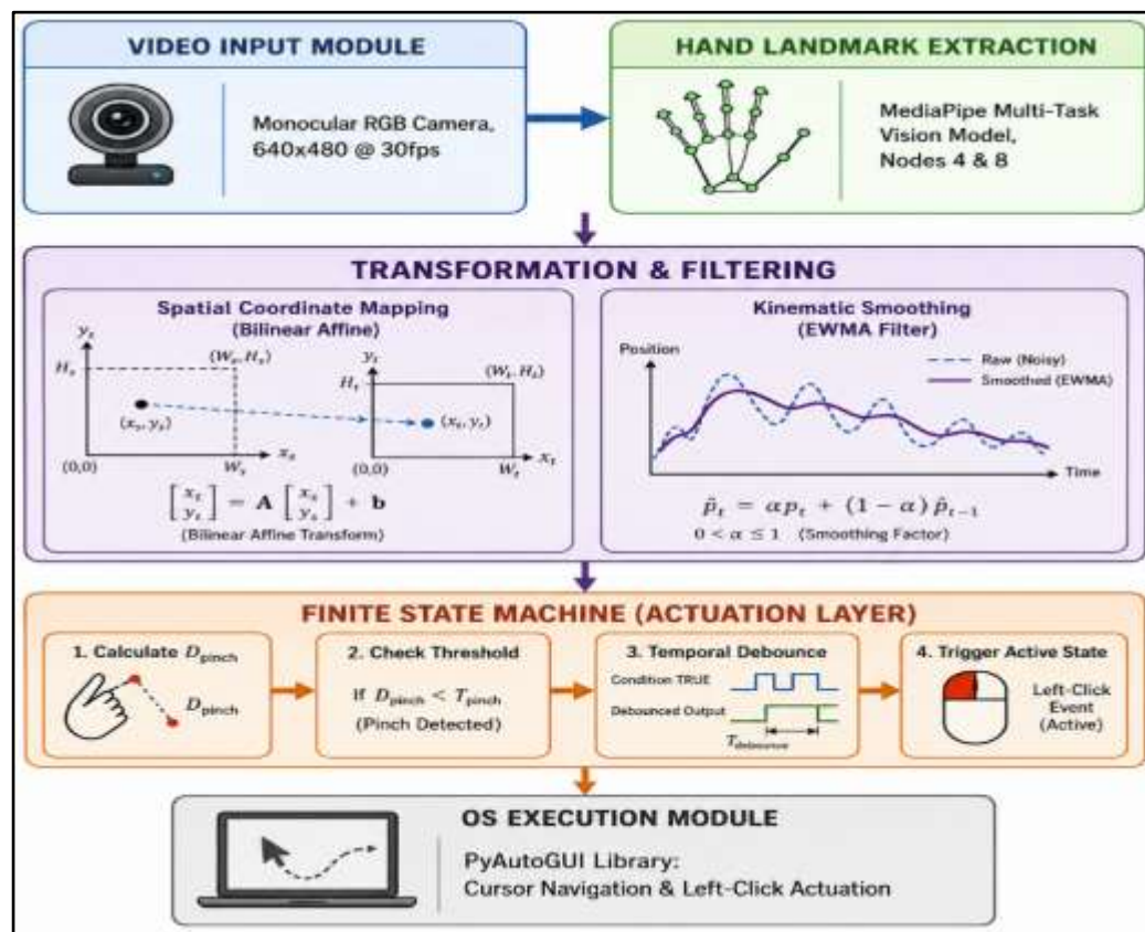
Figure.1. AI Virtual Mouse Control Architecture
