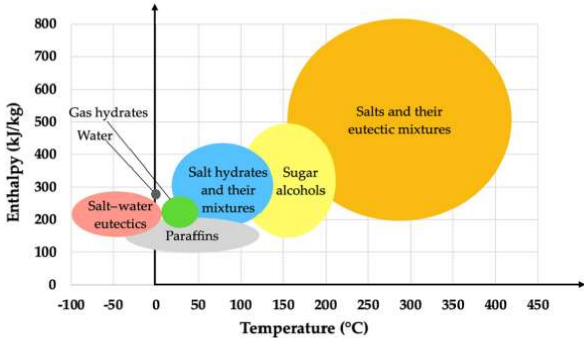
Figure 3 – Plot of working temperature vs. enthalpy of main existing PCMs [26]
