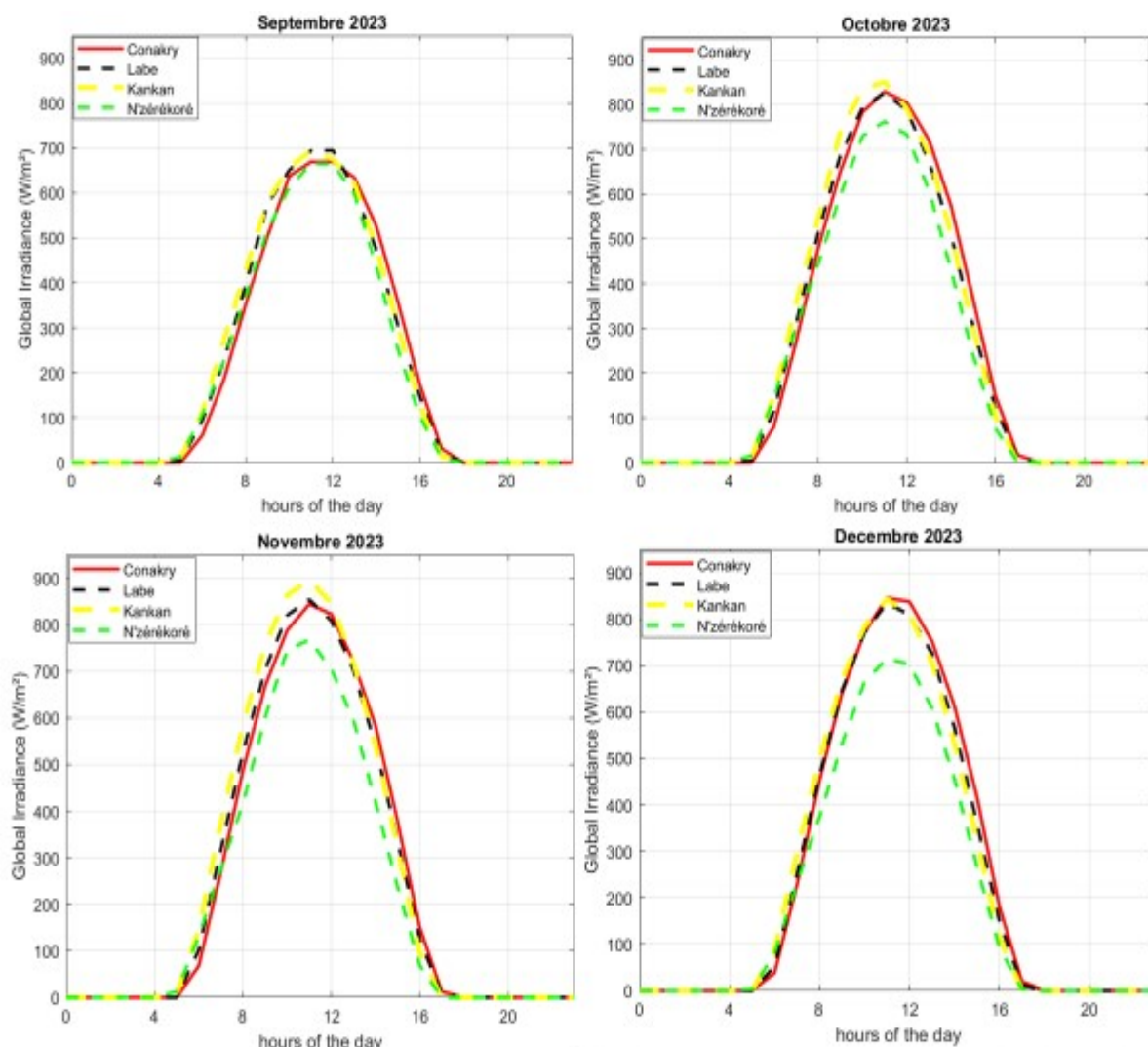
Figure 4: Trends in hourly solar radiation (daily average)
