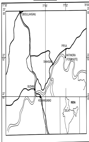
LOCALLY MAP OF NARMADA MAN FOSSIL
