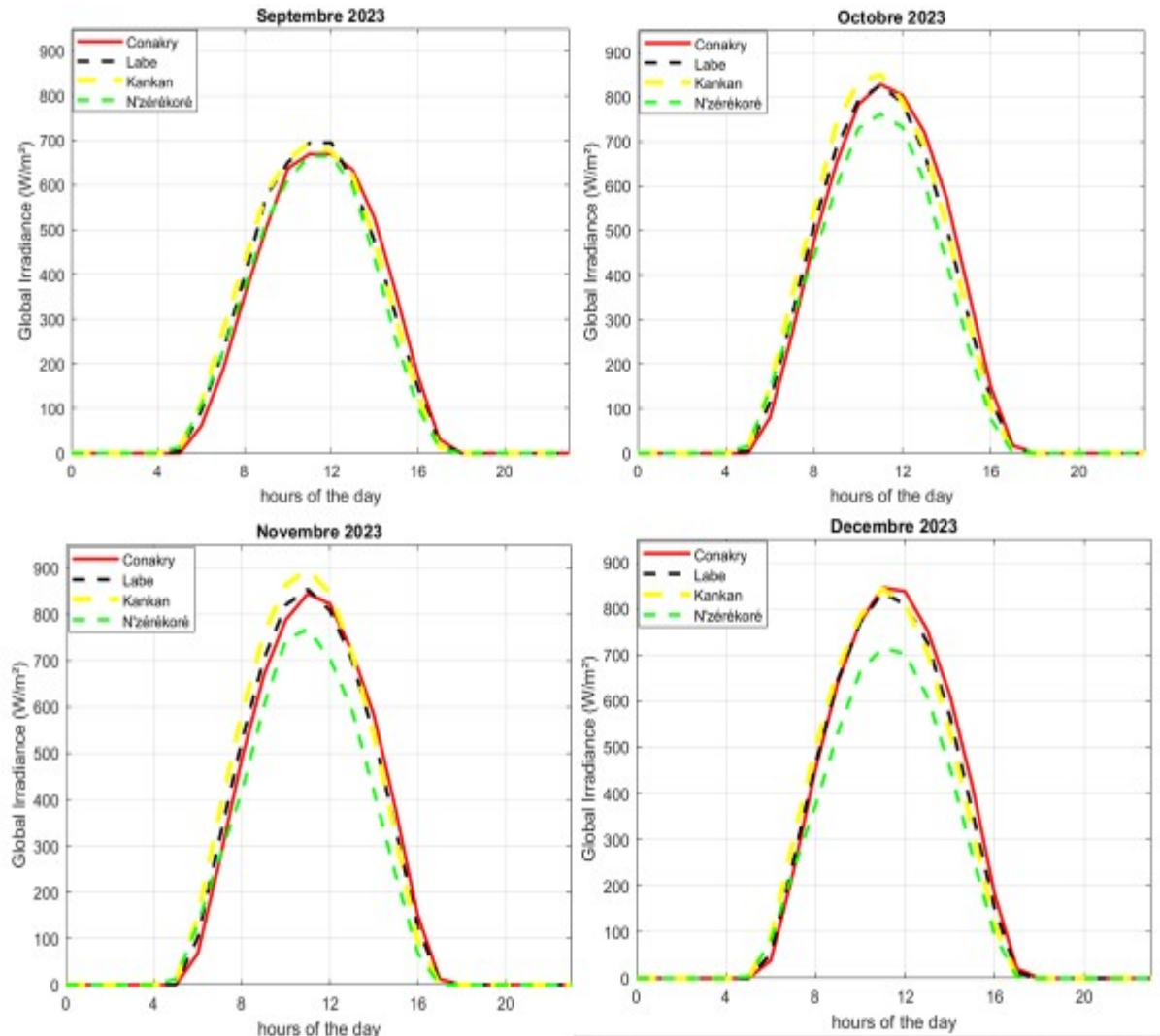
Figure 4: Trends in hourly solar radiation (daily average)
