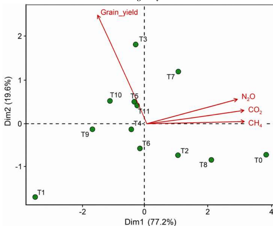
Figure 2. Principal component analysis (PCA) biplot of reductions in greenhouse gas emissions, grain yield, and fertilizer treatments. CH 4 , methane; CO 2 , carbon dioxide; N 2 O, nitrous oxide. T0 = control; T1 = 300 \text{ kg ha}^{-1} NPK + 150 \text{ kg ha}^{-1} urea; T2 = 30 \text{ t ha}^{-1} cattle dung compost; T3 = 30 \text{ t ha}^{-1} cattle dung compost + 50 \text{ kg ha}^{-1} urea; T4 = 30 \text{ t ha}^{-1} cattle dung compost + 175 \text{ kg ha}^{-1} NPK; T5 = 20 \text{ t ha}^{-1} cattle dung compost + 50 \text{ kg ha}^{-1} urea; T6 = 20 \text{ t ha}^{-1} cattle dung compost + 175 \text{ kg ha}^{-1} NPK; T7 = 15 \text{ t ha}^{-1} cattle dung compost + 50 \text{ kg ha}^{-1} urea; T8 = 15 \text{ t ha}^{-1} cattle dung compost + 175 \text{ kg ha}^{-1} NPK; T9 = 30 \text{ t ha}^{-1} cattle dung compost + 175 \text{ kg ha}^{-1} NPK + 50 \text{ kg ha}^{-1} urea; T10 = 20 \text{ t ha}^{-1} cattle dung compost + 175 \text{ kg ha}^{-1} NPK + 50 \text{ kg ha}^{-1} urea; T11 = 15 \text{ t ha}^{-1} cattle dung compost + 175 \text{ kg ha}^{-1} NPK + 50 \text{ kg ha}^{-1} urea.
