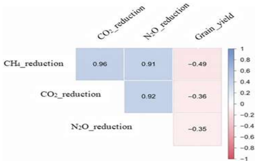
Figure 1. Pearson correlation matrix between greenhouse gas emission reductions (CH 4 , CO 2 and N 2 O) and rice grain yield.
