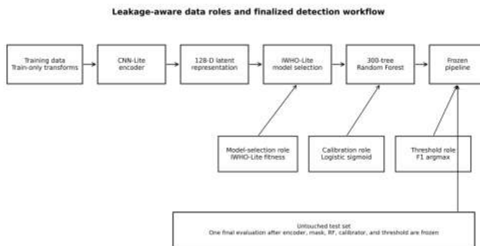
Fig. 2. Leakage-aware data roles and final detection workflow. Fitted preprocessing is confined to the training scope. The model-selection role also supports CNN-Lite training control and early stopping; the arrow to IWHO-Lite highlights its use for mask fitness. Logistic mapping and fixed-threshold selection use dedicated downstream validation roles. Final testing occurs only after the encoder, latent mask, Random Forest, calibrator, and threshold have been frozen.
