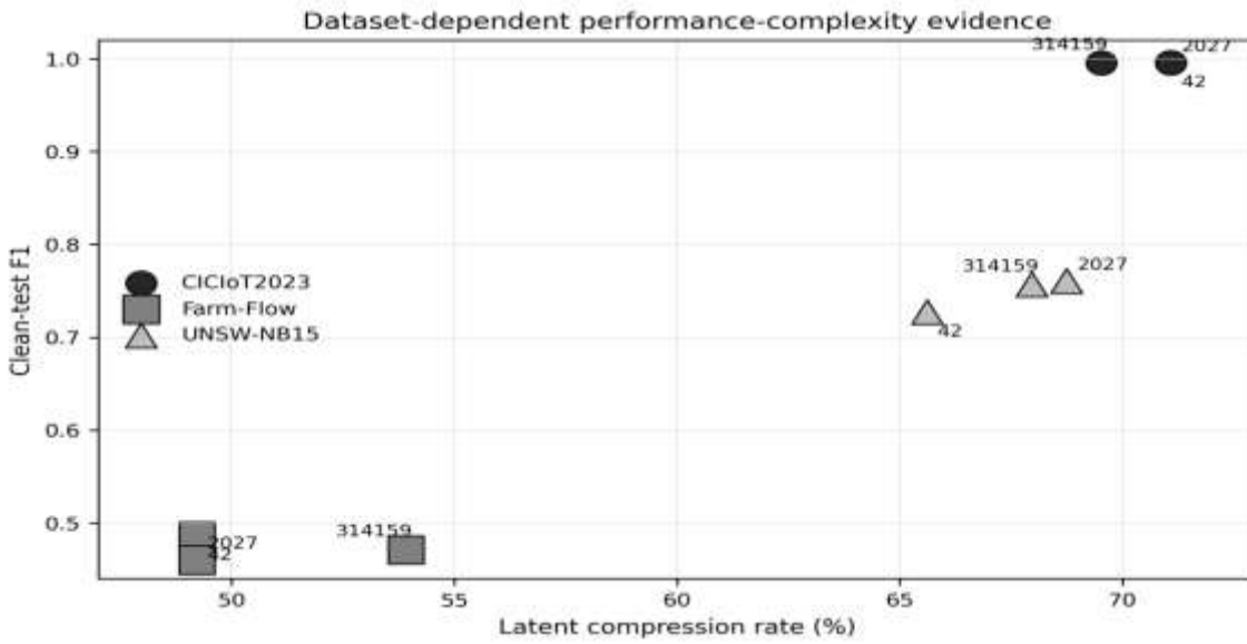
Fig. 3. Clean-test F1 versus latent compression. Each point represents an individual dataset-seed run; marker area reflects measured batch latency. The plot is descriptive and does not define a Pareto frontier. Marker size should not be interpreted as an energy or hardware-efficiency measurement.
