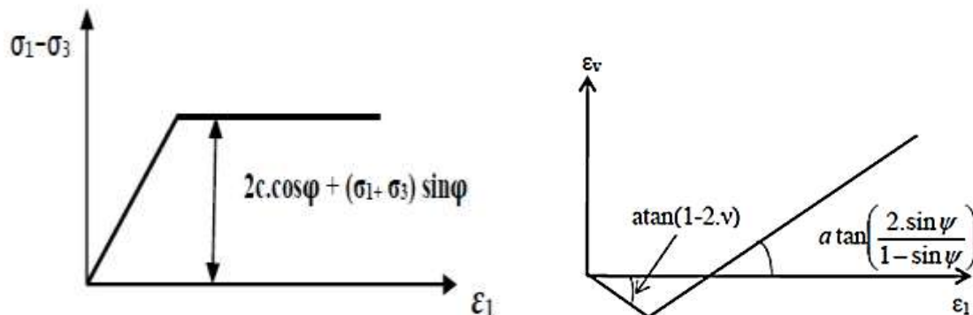
Figure 8. Mohr-Coulomb model.
