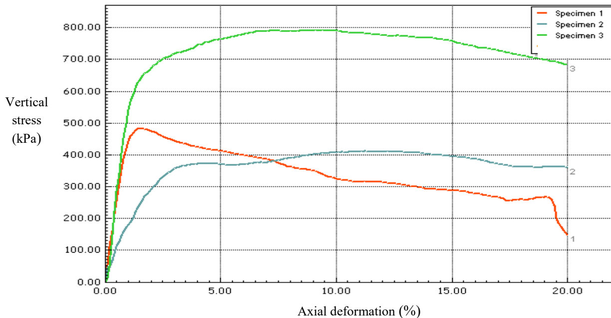
Figure 10. Stress-strain curve for the raw lateritic gravel.
