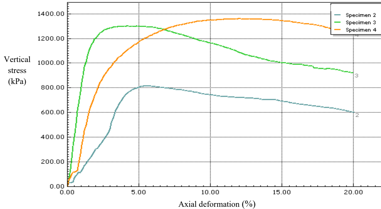
Figure 12. Stress-strain curve for the lateritic gravel reinforced with 0.75% jute fibers -1 cm.
