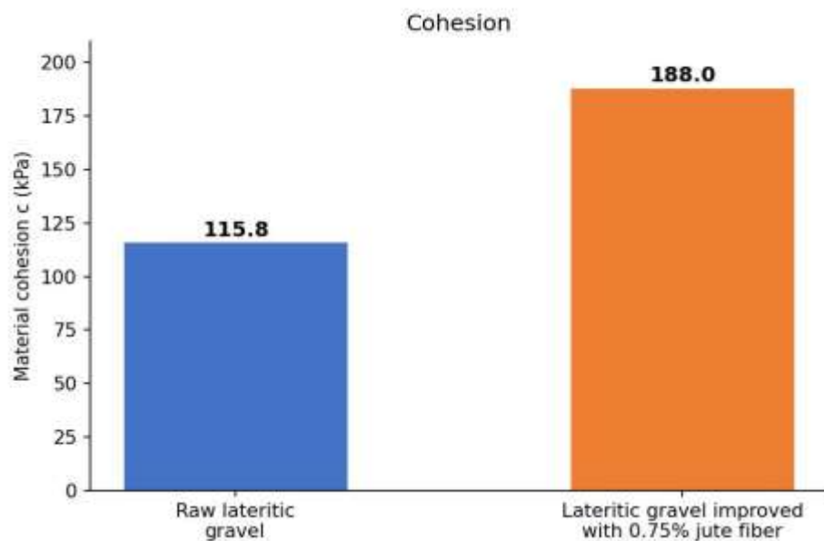
Figure 13. Variation of material cohesion.
