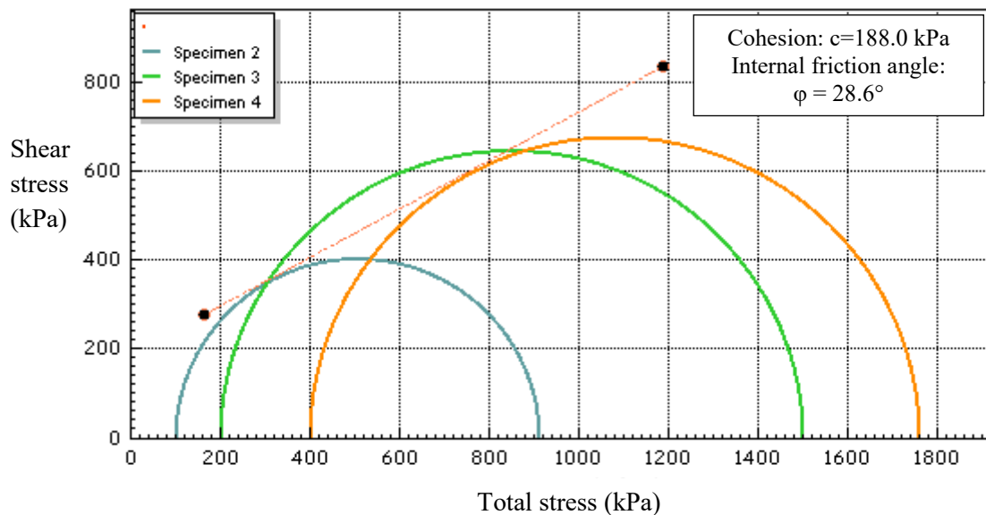
Figure 11. Shear stress–total stress curves for the lateritic gravel reinforced with 0.75% jute fibers -1 cm (UU test, total stresses).
