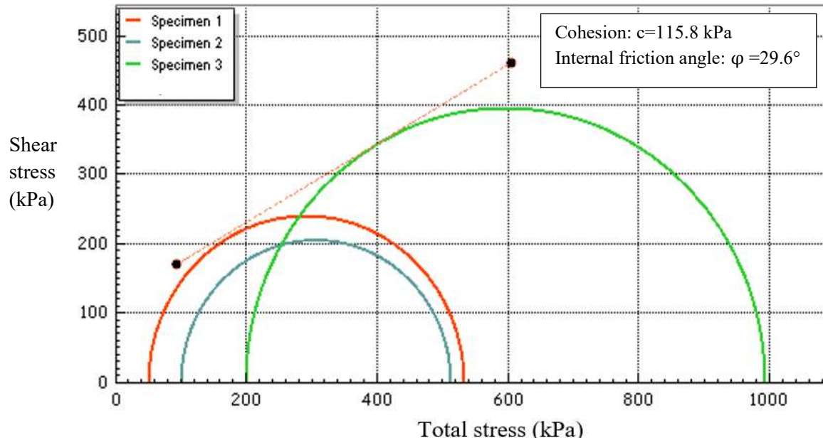
Figure 9. Shear stress–total normal stress curves for the raw lateritic gravel (UU test, total stresses).
