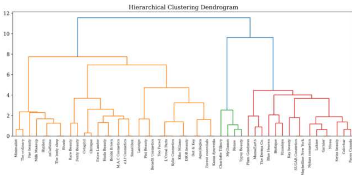
Figure 4: Dendrogram Analysis of brand clustering based on shared inclusivity philosophies Source: Author's own creation using Python
