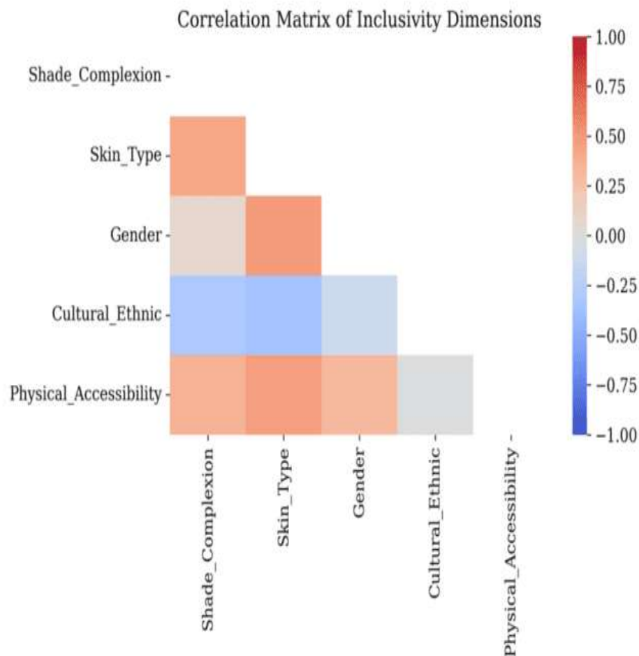
Figure 1: Correlation heatmap illustrating interconnectivity and trade-offs among Brand Inclusivity Dimensions
