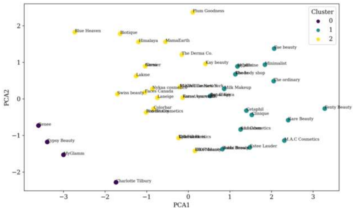
Figure 3: Two-dimensional PCA projection mapping Brand Positions across inclusivity cluster segments Source: Author's own creation using Python
