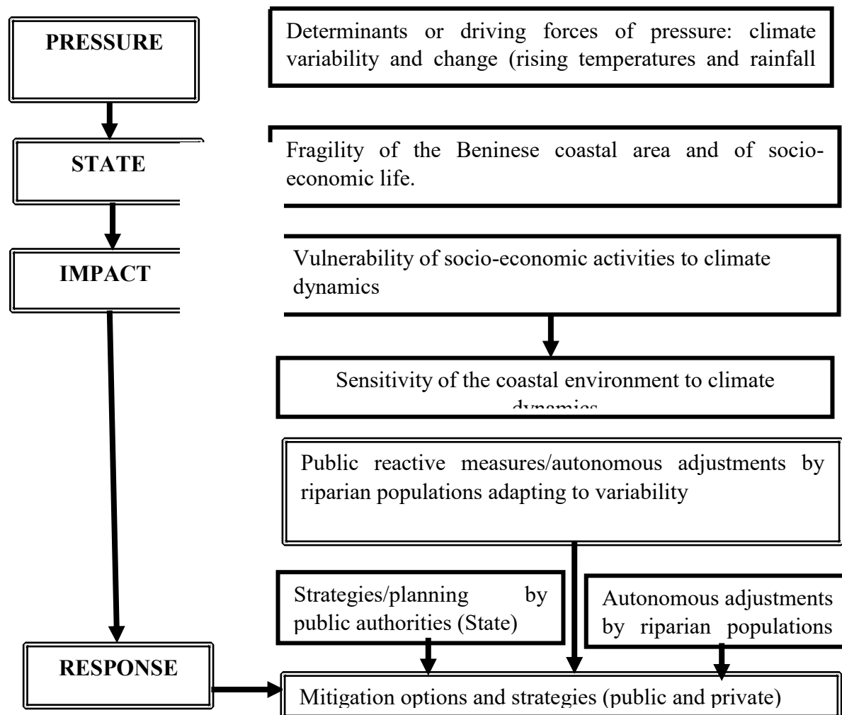
Figure 2: Analytical model of the links between climate, socio-economic activities, and natural resources
