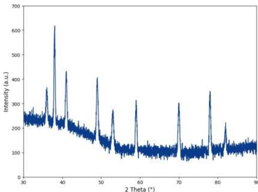
Figure 3. XRD pattern of the synthesized G-AgNPs using Garlic ( Allium sativum ) leaf extract
