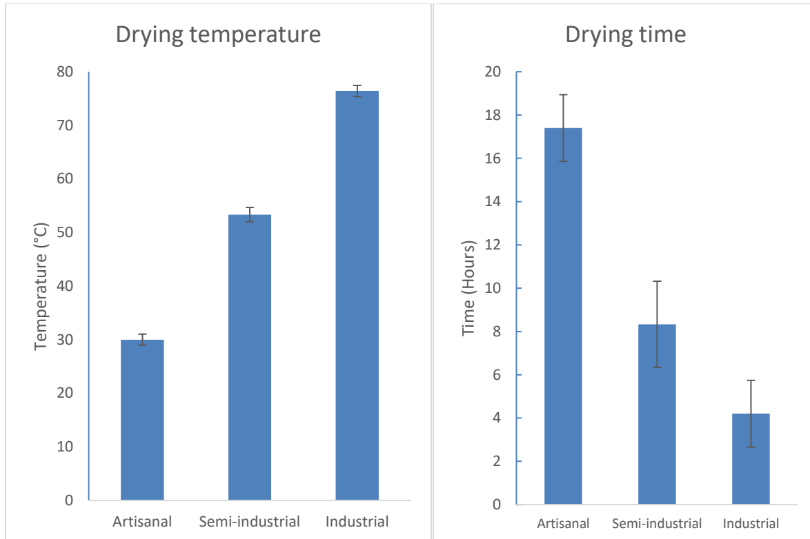
Figure 1. Temperature and time used in the surveyed cashew nut processing systems
