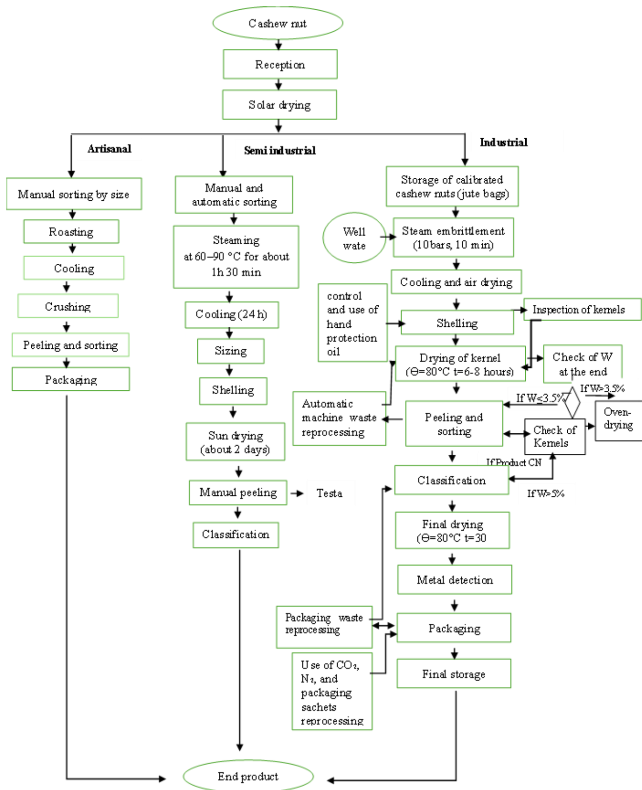
Figure 2: Flow sheet of cashew nut production process system
