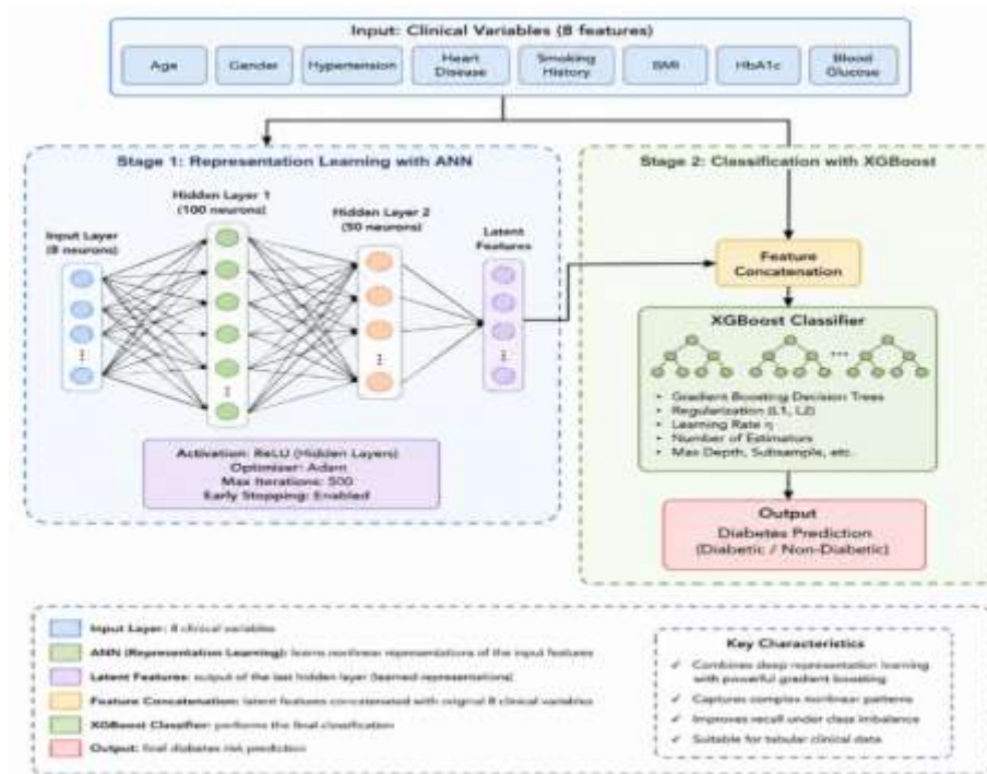
Figure 3. Hybrid ANN–XGBoost Architecture
