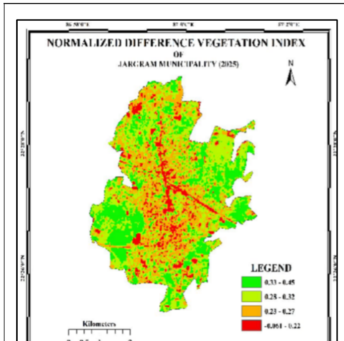
Fig: 2.7 NDVI of Jhargram Municipality (2025)
