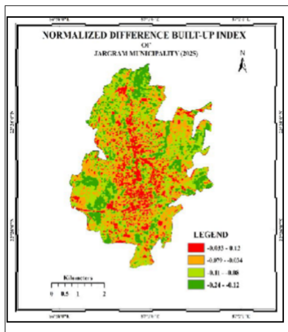
Fig: 2.6 NDBI of Jhargram Municipality (2025)
