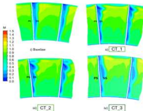
Figure 15. Variation of Relative Mach Number on Streamwise Plane-1 At Near Design Mass Flow Rate Of 20.188 Kg/S: (A) Baseline Stage, (B) Casing Treated Stage Case Ct-1, And (C) Casing Treated Stage Case Ct-2 And (D) Casing Treated Stage Case Ct-3
