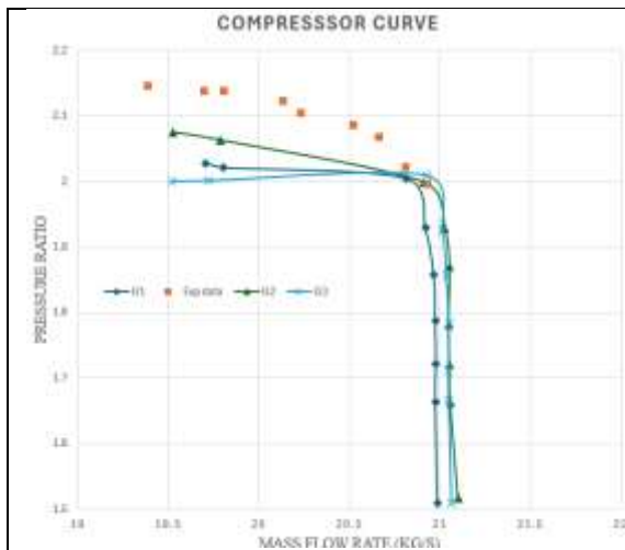
Figure.6 Grid Independence Study – Variation of Total Pressure Ratio with Mass Flow Rate
