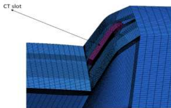
Figure 9: Computational Grid for Compressor Stage with Casing
