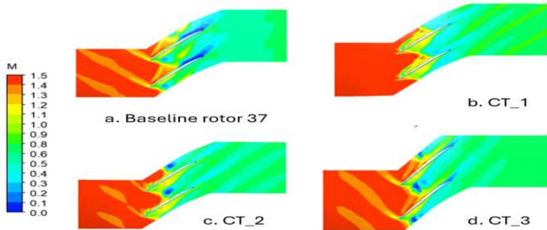
Figure 12. Mach Counter Plots at Stall Operating Point
