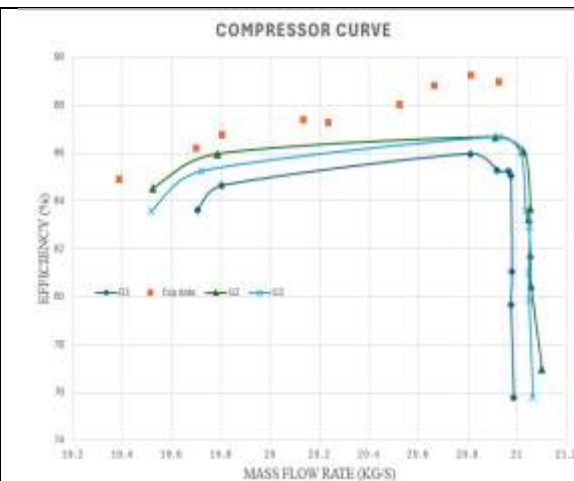
Figure.7 Grid Independence Study – Variation of Efficiency with Mass Flow Rate
