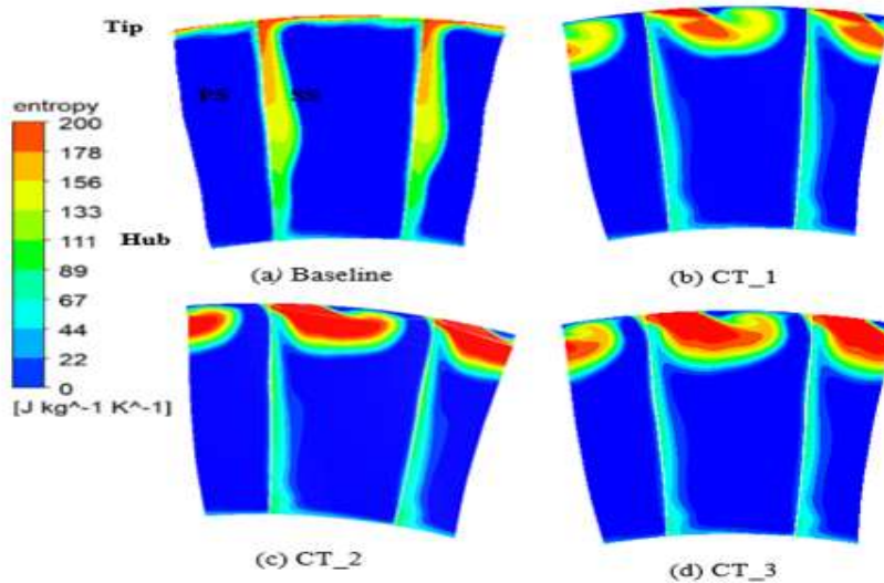
Figure 14. Variation of Entropy at Stream Wise Plane-2 At Mass Flow Rate Equal to Stall Mass Flow Rate: (A) Baseline Stage, (B) Casing Treated Stage Case Ct-1, (C) Casing Treated Stage Case Ct-2 And (D) Casing Treated Stage Case Ct-3
