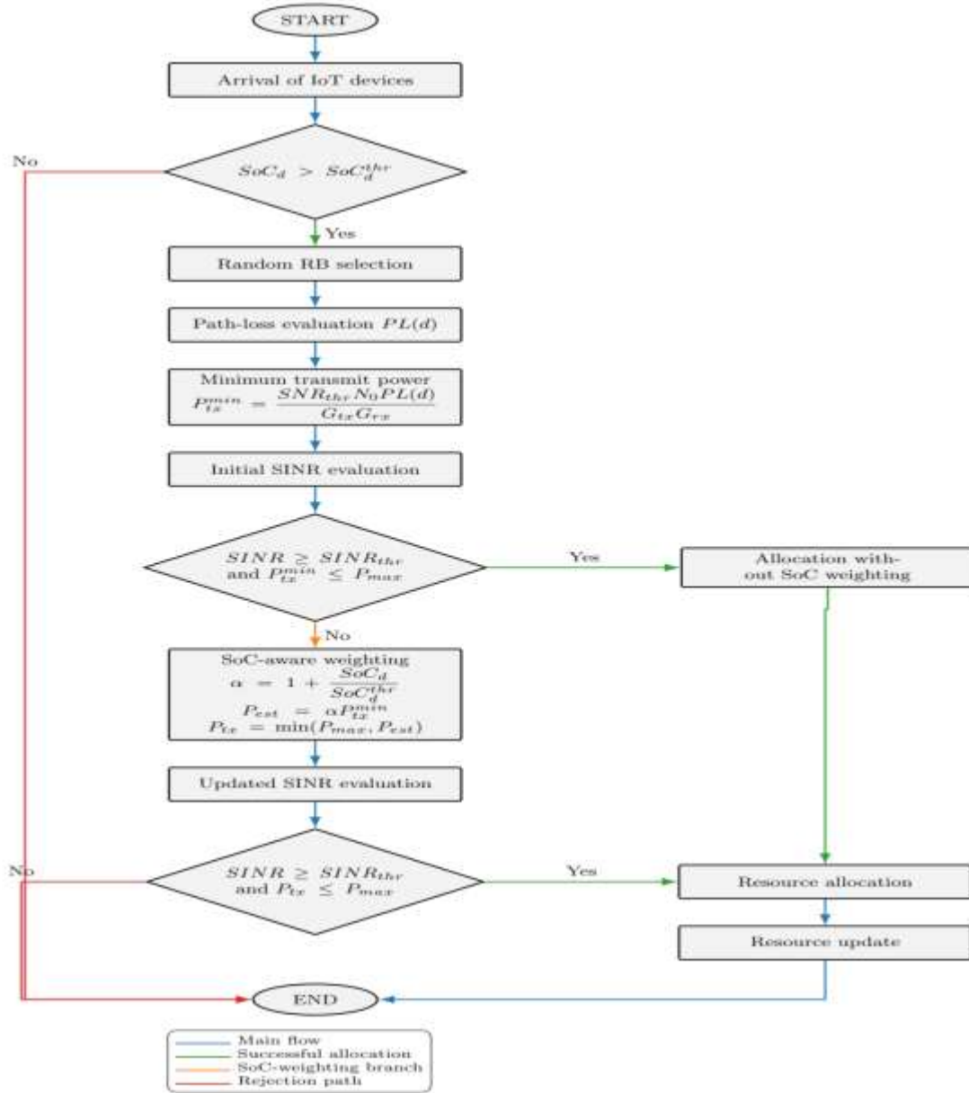
Figure 2. Proposed SoC-aware heuristic resource allocation algorithm for IoT.
