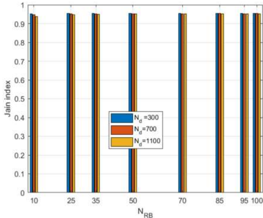
Figure 4. Jain fairness index of IoT users.
