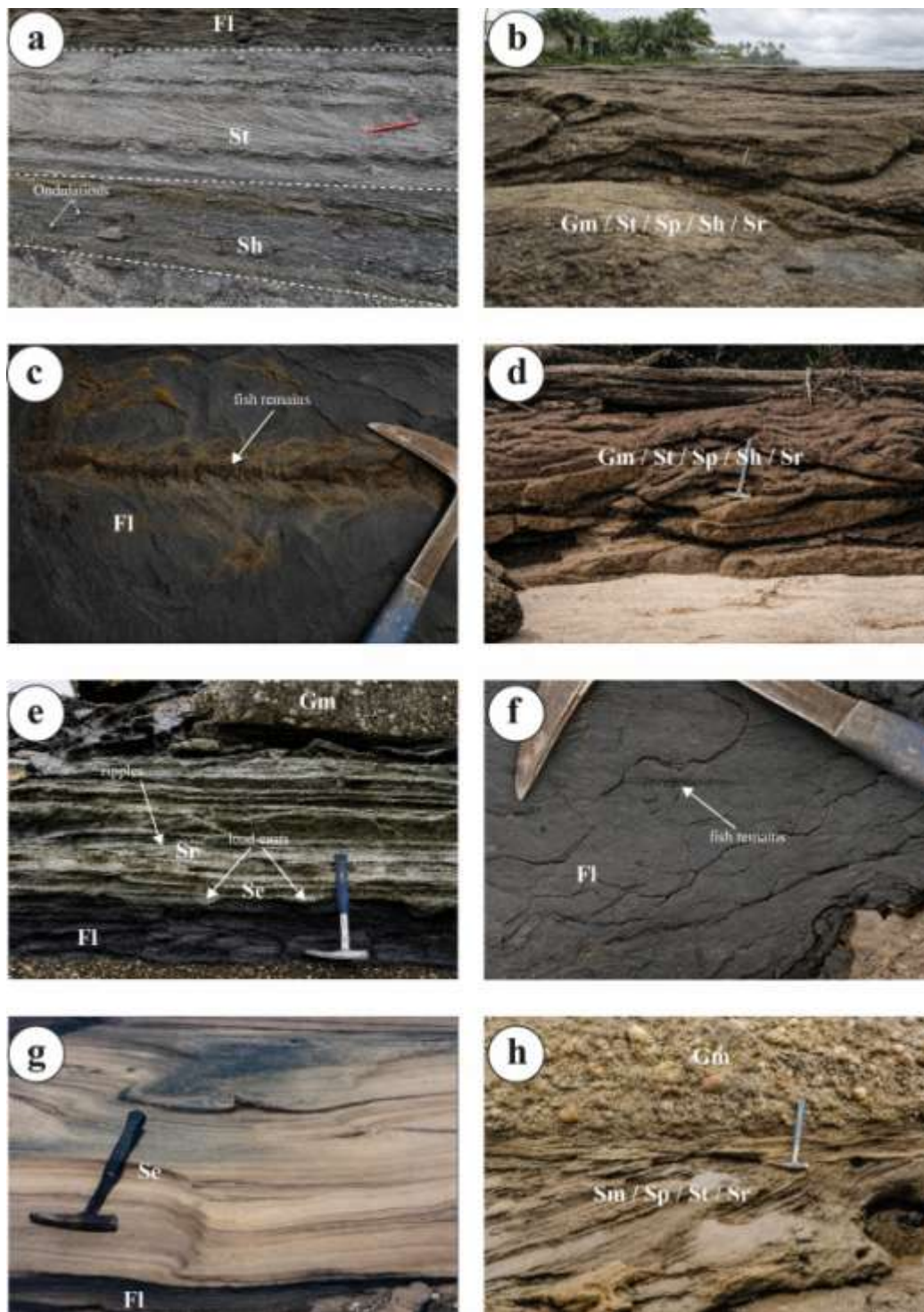
Fig. 4. Sedimentary lithofacies types from theCocobeachBeach section: a) Bed 1,b,d) Bed 2,c) Bed 3,e-g) Bed 6,h) Bed 8.
