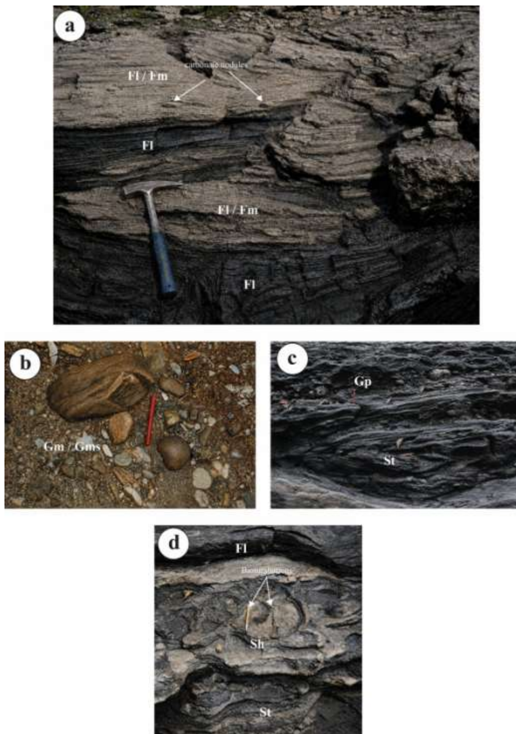
Fig. 6. Sedimentary lithofacies types: a) from the Cocobeach Southern Landing Stage section; b) Bed 5, c) Bed 7, d) Bed 4, from the the South of the Cocobeach Quay Lighthouse section.
