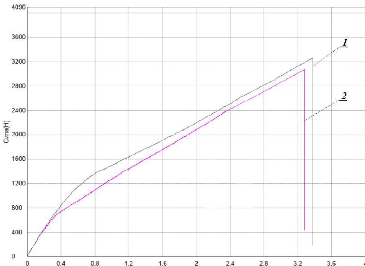
Figure 2. Stress-strain curves under tension for epoxy polymers:
