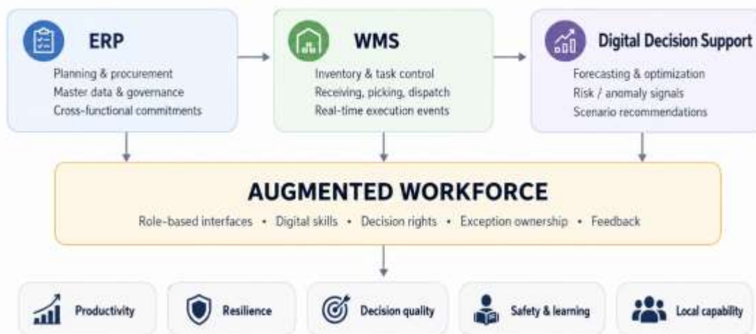
Figure 1. Integrated ERP-WMS-DDS architecture for workforce augmentation.
