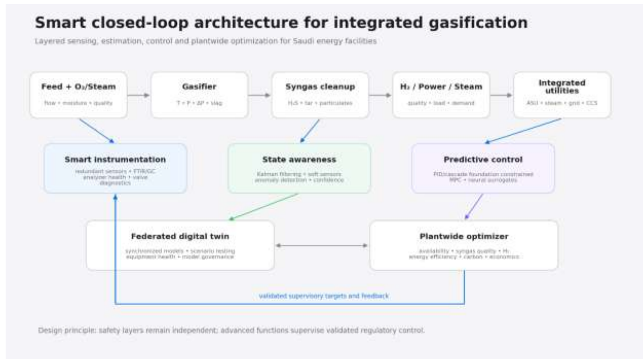
Figure 1. Smart closed-loop architecture for integrated gasification
