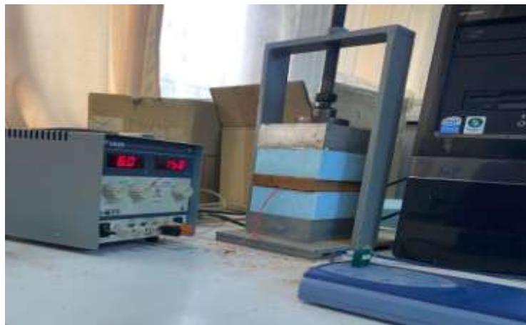
Figure 8:-Conductivity measuring device
