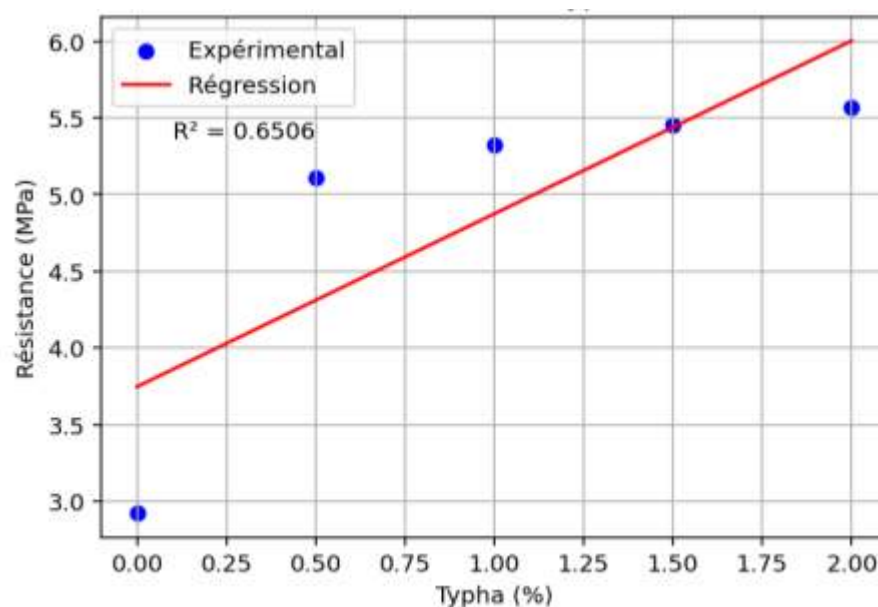
Figure 13:-Compressive strength as a function of typha content.
