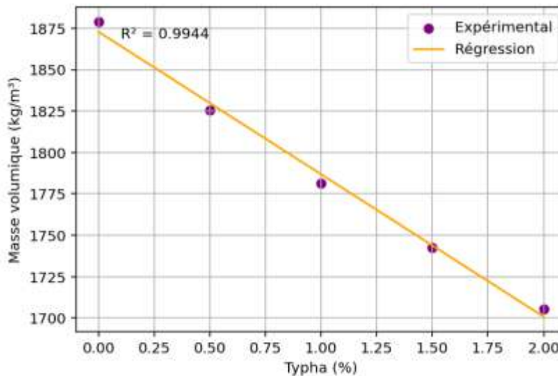
Figure 11:-Density as a function of the percentage of typha
