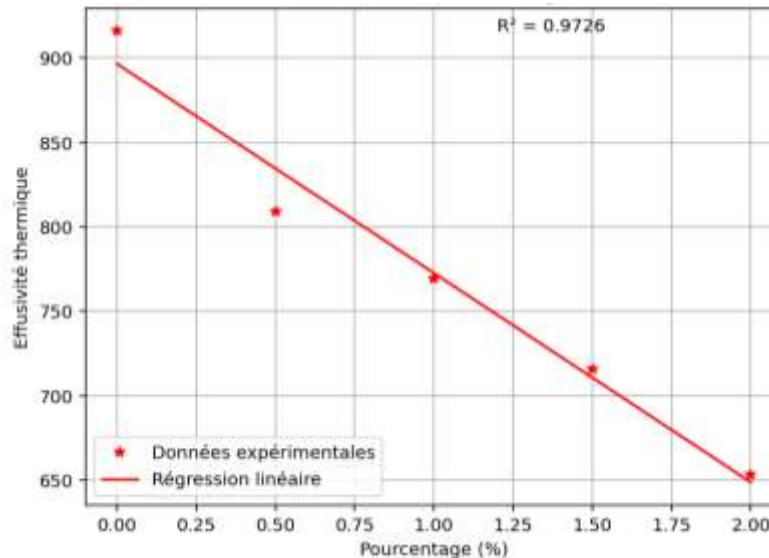
Figure 14:-Thermal effusivity as a function of the percentage of typha
