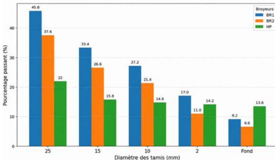
Figure 9:-Typha grain size histogram
