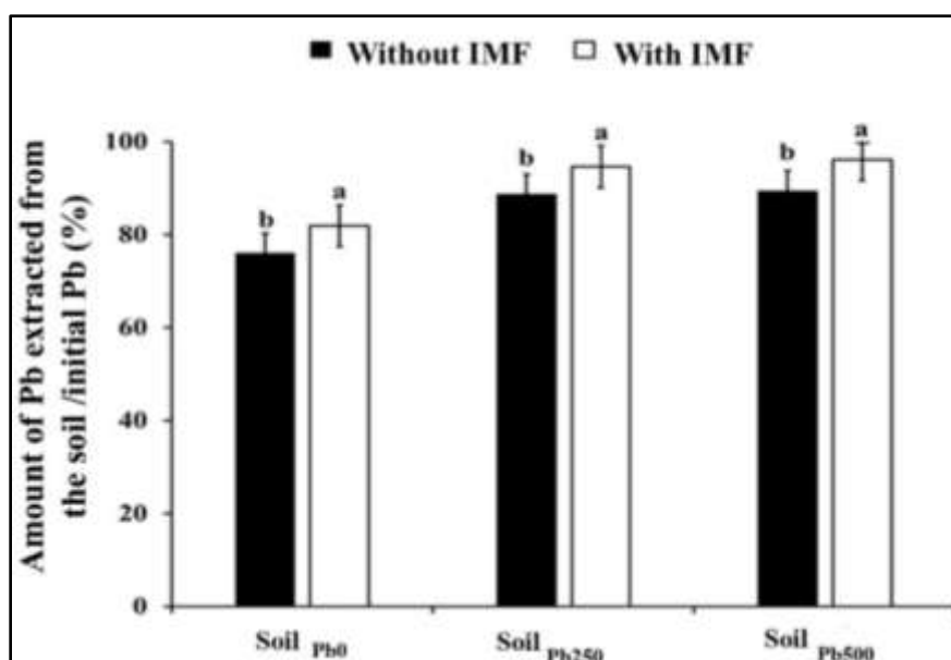
Figure 3: Proportion of Pb extracted from the soil (%) after phytoremediation, relative to the initial Pb content. Soil Pb_0 : Non-contaminated soil; Soil Pb_{250} : Soil contaminated with lead 250 mg/kg; Soil Pb_{500} : Soil contaminated with lead 500 mg/kg; IMF: Indigenous arbuscular mycorrhizal fungi. The histograms followed by the same letter (a, b) are not significantly different according to the Newman-Keuls Student's test at P < 0.05 .
