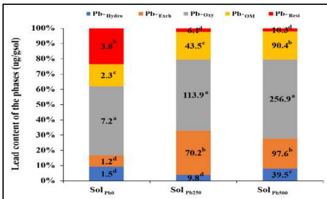
Figure 2: Fractionation of lead (Pb) before phytoremediation
