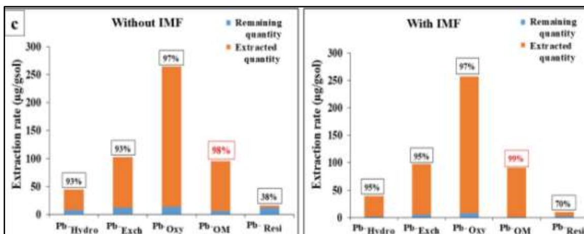
Figure 4: Extraction rate of lead content ( \mu\text{g/gsoil} ) under the different studied soils (Soil Pb0 (a), Soil Pb250 (b), Soil Pb500 (c)) in the absence (Without IMF) and presence (With IMF) of fungal isolates after five months of phytoremediation of the different fractions.
