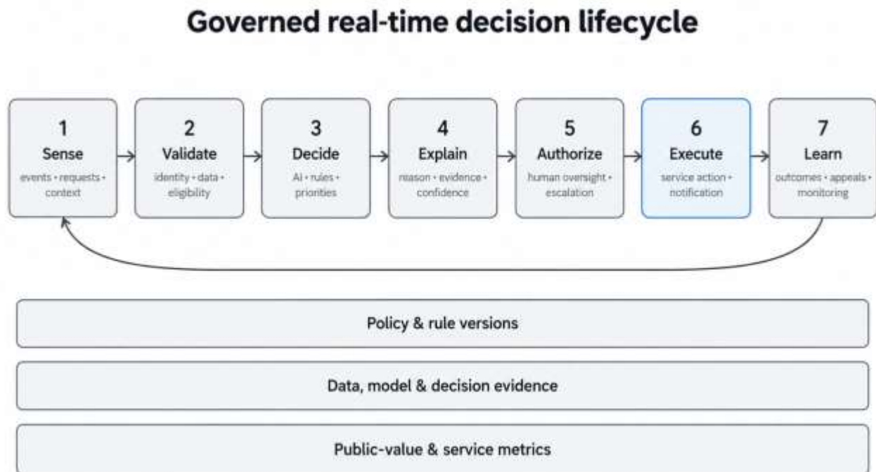
Figure 2. Governed real-time decision lifecycle with continuous evidence and public-value controls.
