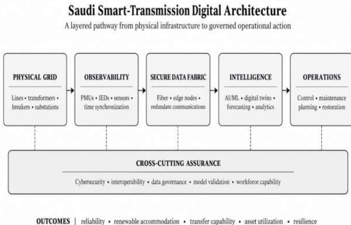
Figure 1. Layered smart-transmission architecture linking physical assets, observability, secure data infrastructure, analytics and governed operations. Source: synthesis developed in this review.
