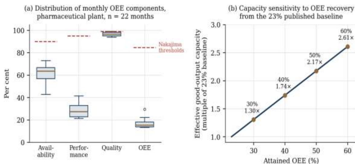
Figure 2. (a) Distribution of monthly OEE components across twenty-two reported months at a pharmaceutical plant, plotted against Nakajima's world-class component thresholds; recomputed from the published series in Chikwendu et al. (2020), Heliyon , 6(4), e03796. (b) Effective good-output capacity as a multiple of the 23 per cent baseline reported by Zubair et al. (2021), Cogent Engineering , 8(1), 1953681.
