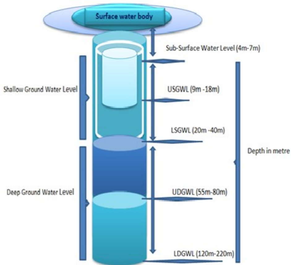
Fig: 1 Positioning places of water sources
