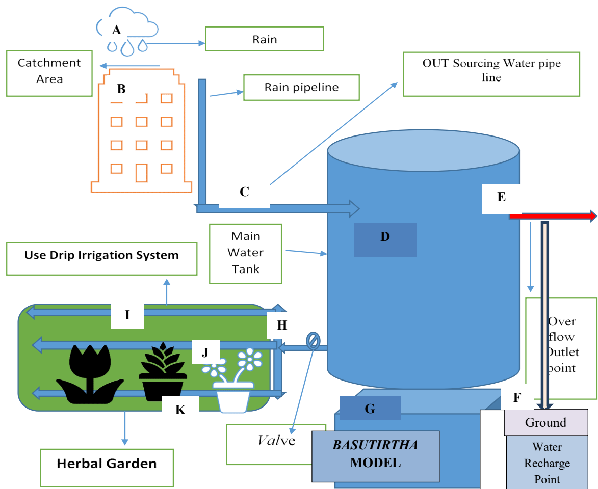
Fig 2: Model of Basutirtha Rain water harvesting with micro irrigation technology
