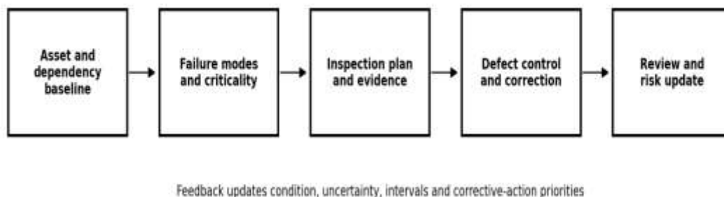
Figure 1. Integrated risk-based electrical inspection and quality-control cycle.
