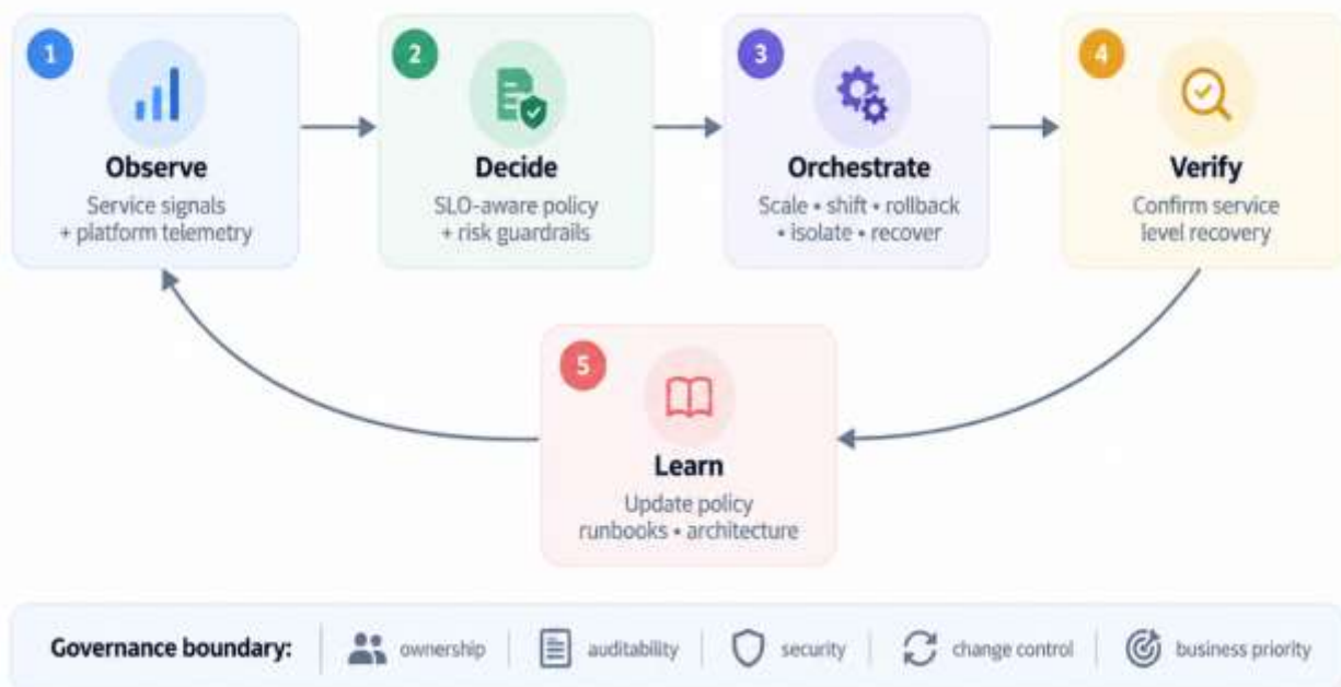
Figure 2. Closed-loop model linking observability, bounded automation, verification and governance.
