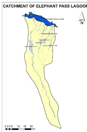
Figure 2.1: Catchment of Elephant Pass lagoon
