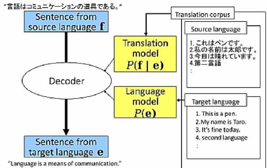
Fig 6:- SMT Framework.
