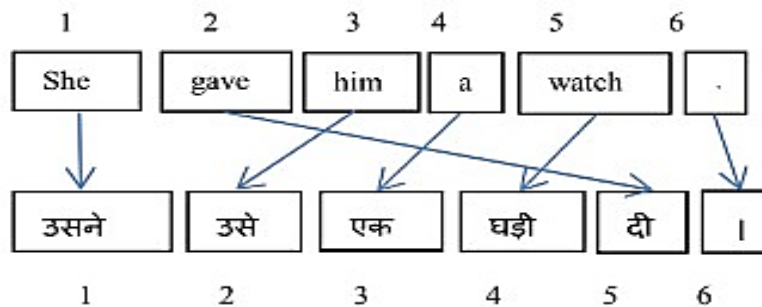
Fig 2:- Example 2.
