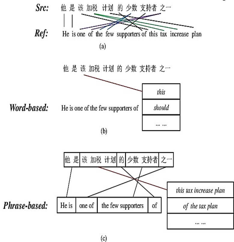
Fig 5:- Translation.
