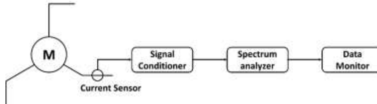
Figure (2):- Motor current signature analysis chart.
