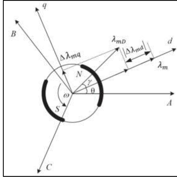
Figure (1):- Variation of the PMSM flux linkage.
