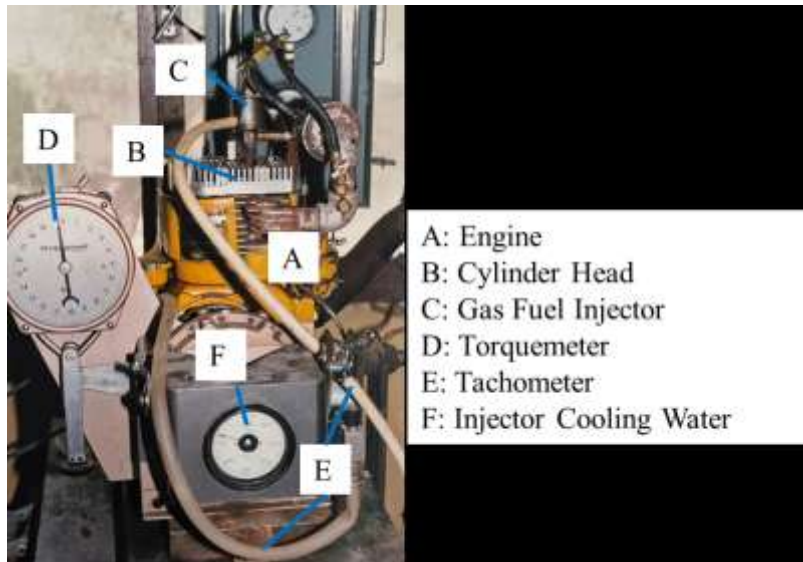
Figure 3:- Single piston ICE, cylinder head, and injector.
