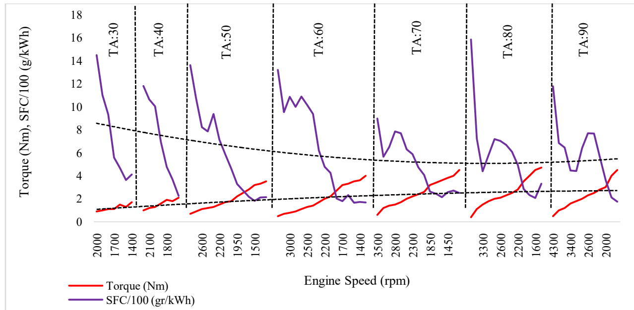
Figure 8:-PICE Engine speed, torque, SFC.
