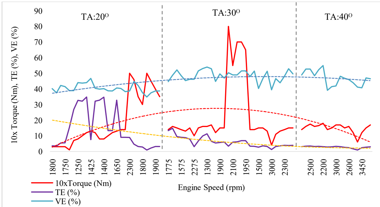
Figure 12:- H 2 ICE Engine speed, torque, TE, VE.
