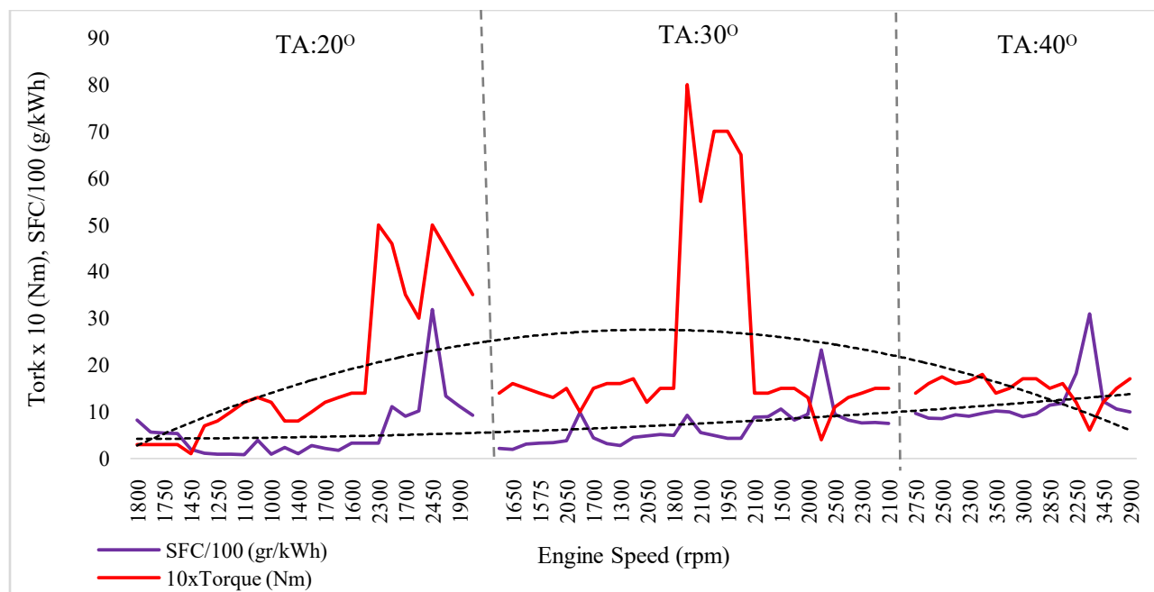
Figure 11:-H 2 ICE Engine speed, torque, SFC.
