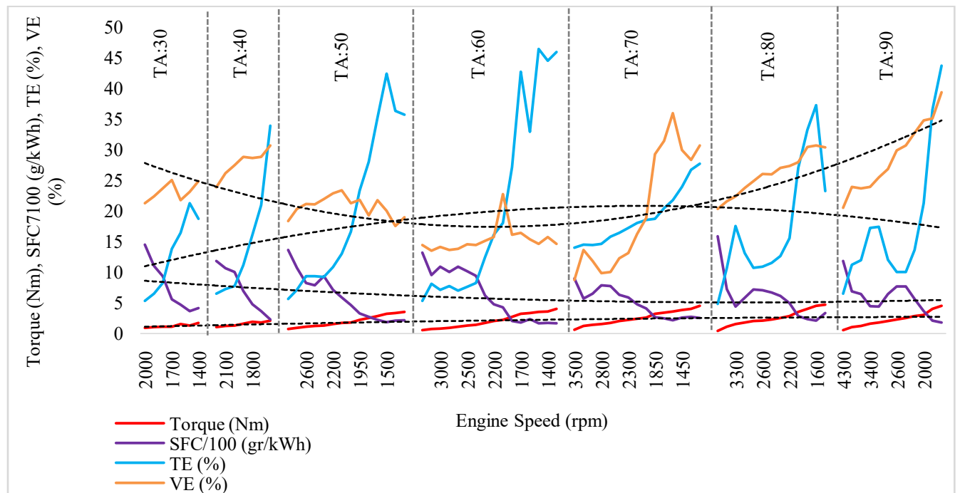
Figure 9:-GICE Engine speed, Torque, SFC, TE, VE.
