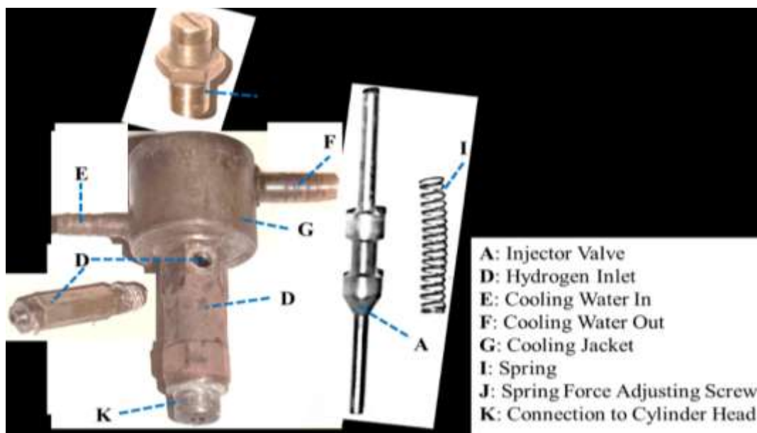
Figure 6:- Mechanically Activated Gas Fuel Injector and main parts.
