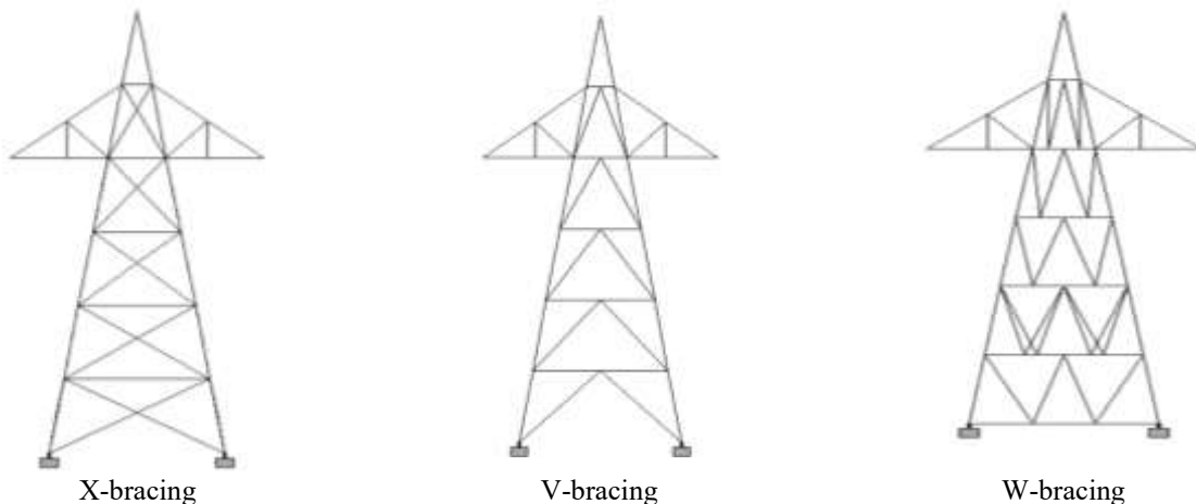
Figure 2 Tower with different bracing systems
