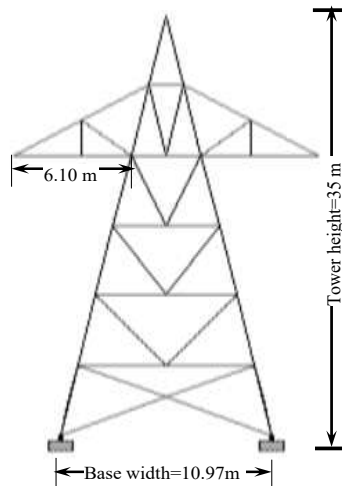
Figure 1 Transmission tower
