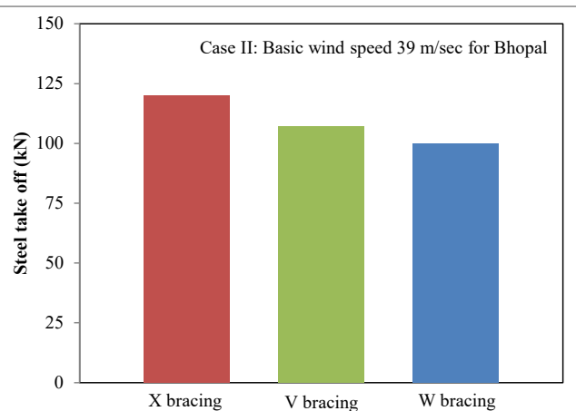
Figure 8 Steel take-off quantities for different bracing systems
