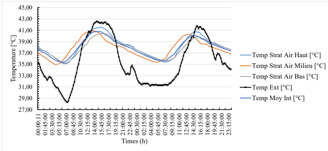
Figure 4: External and internal temperature trends
