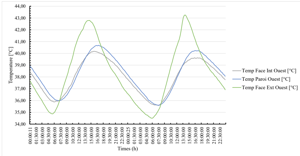
Figure 10: Temperature trends through the west wall
