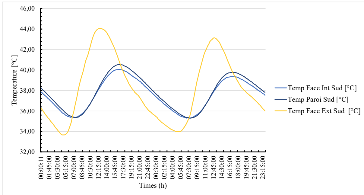
Figure 8: Temperature trends through the south wall
