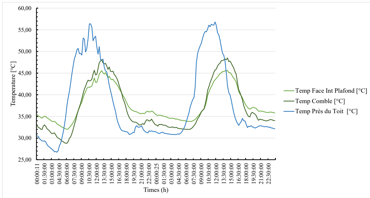
Figure 11: Temperature changes through the roof
