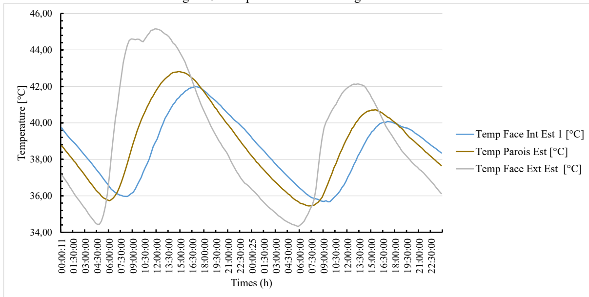
Figure 9: Temperature trends across the east wall
