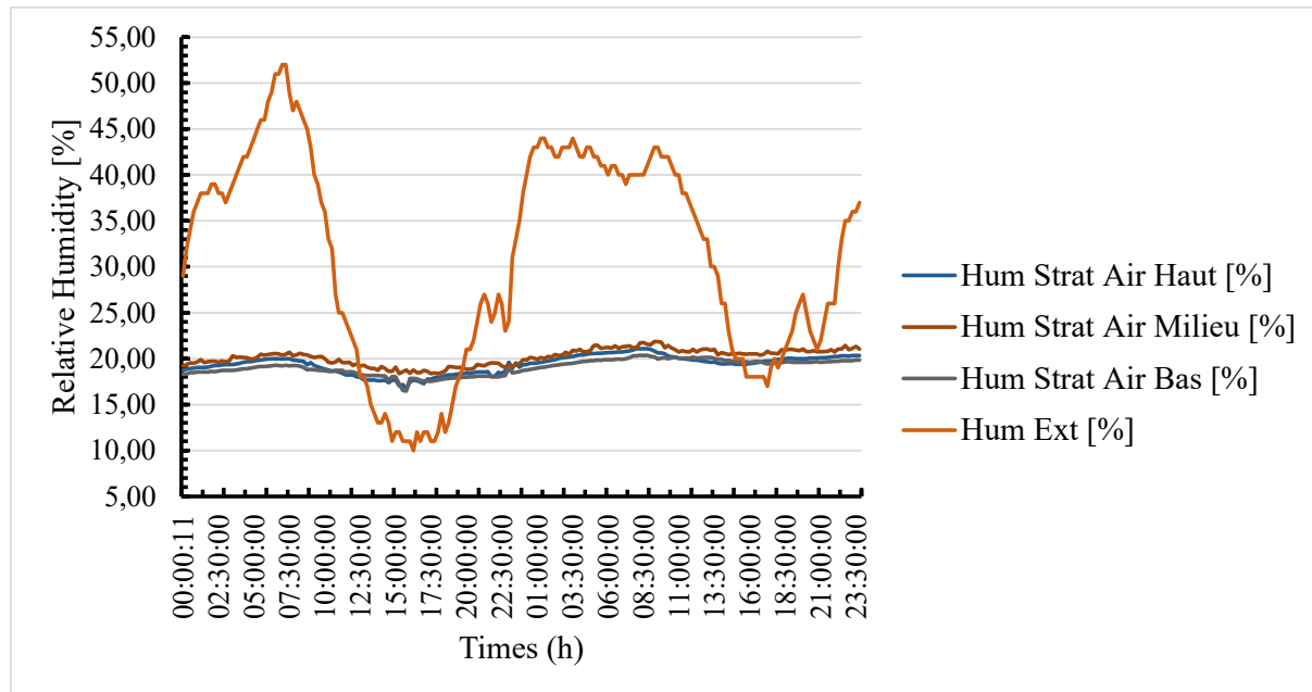
Figure 14: Change in relative humidity
