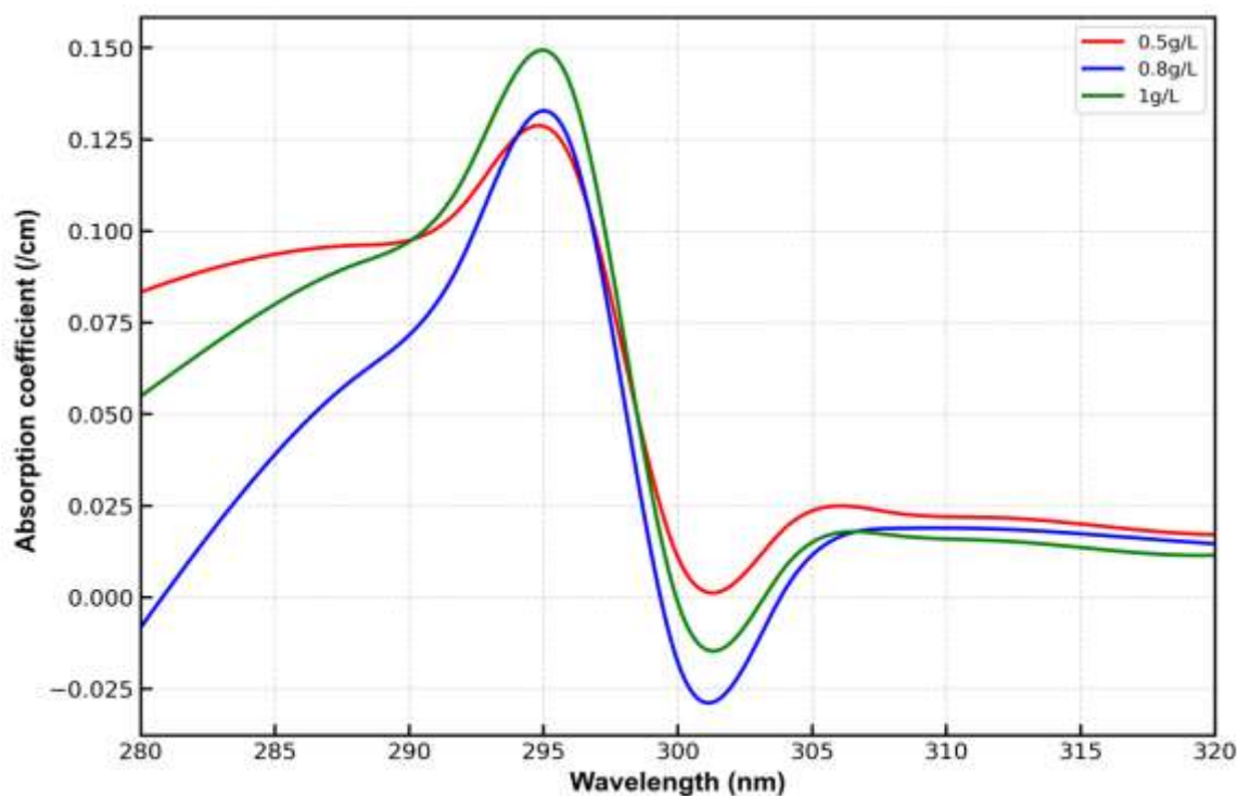
Figure 2:- The relation between the adsorption coefficient and the wavelengths for different concentration of Polystyrene (PS) microplastic.
