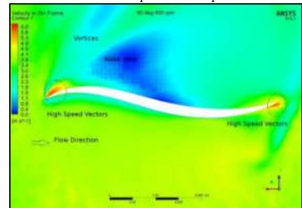
Fig. 7. (f):- Velocity Contour of blade at 90° with a rotational speed of 400 rpm.
