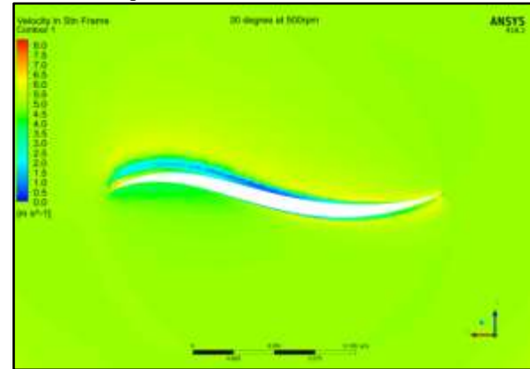
Fig. 7. (b):- Velocity Contour of blade at 30° with a rotational speed of 500 rpm.
