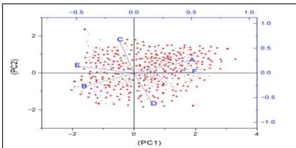
Fig.8:- Variables contribute, with the length of the vectors reflecting their relative importance to the principal components and the angle between any two components reflecting the degree of their association.
