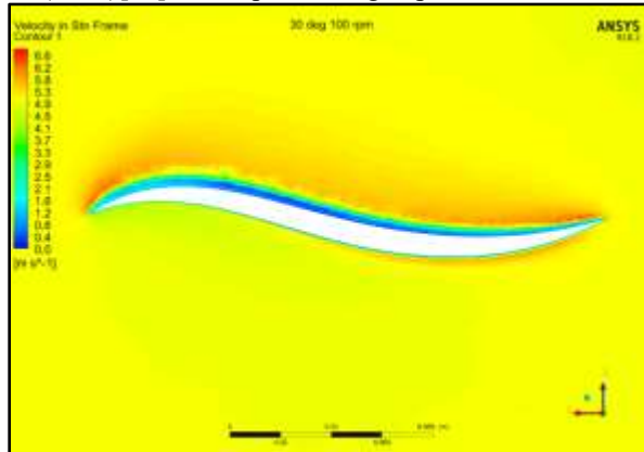
Fig. 7.(a):- Velocity Contour of blade at 30° with a rotational speed of 100 rpm.
