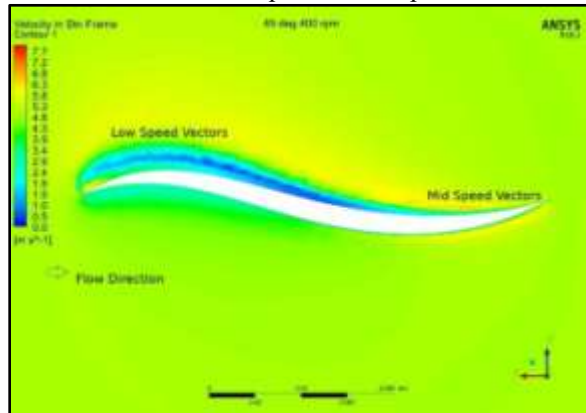
Fig. 7. (c):- Velocity Contour of blade at 45° with a rotational speed of 400 rpm.
