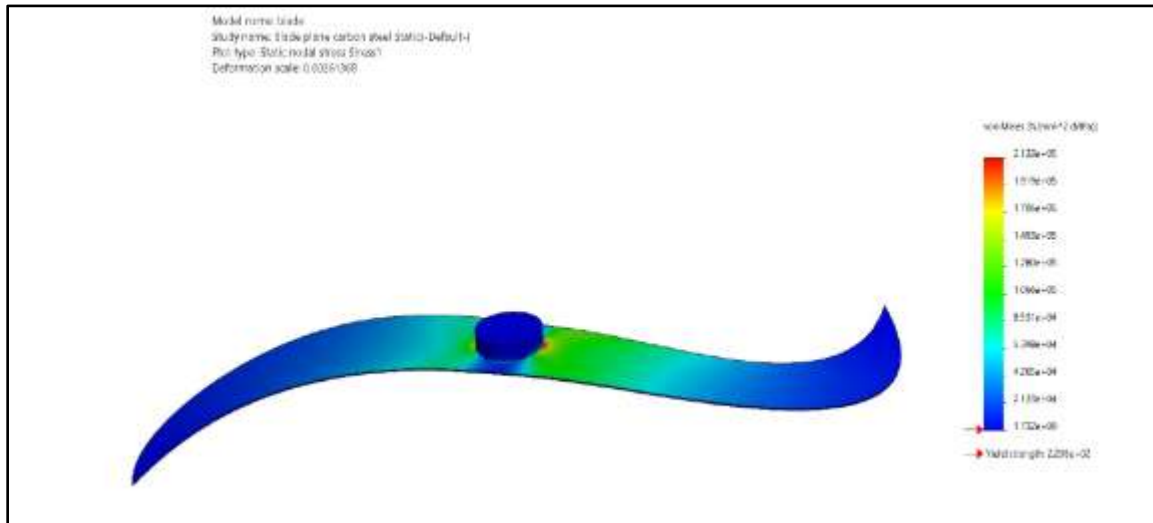
Fig.4:- Static stress plot of plain carbon steel blade.
