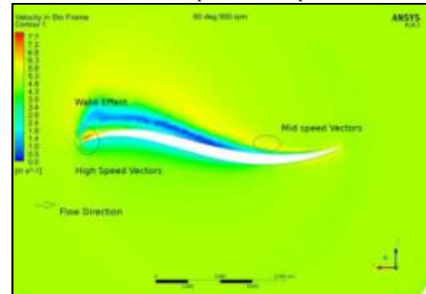
Fig. 7. (d):- Velocity Contour of blade at 60° with a rotational speed of 500 rpm.
