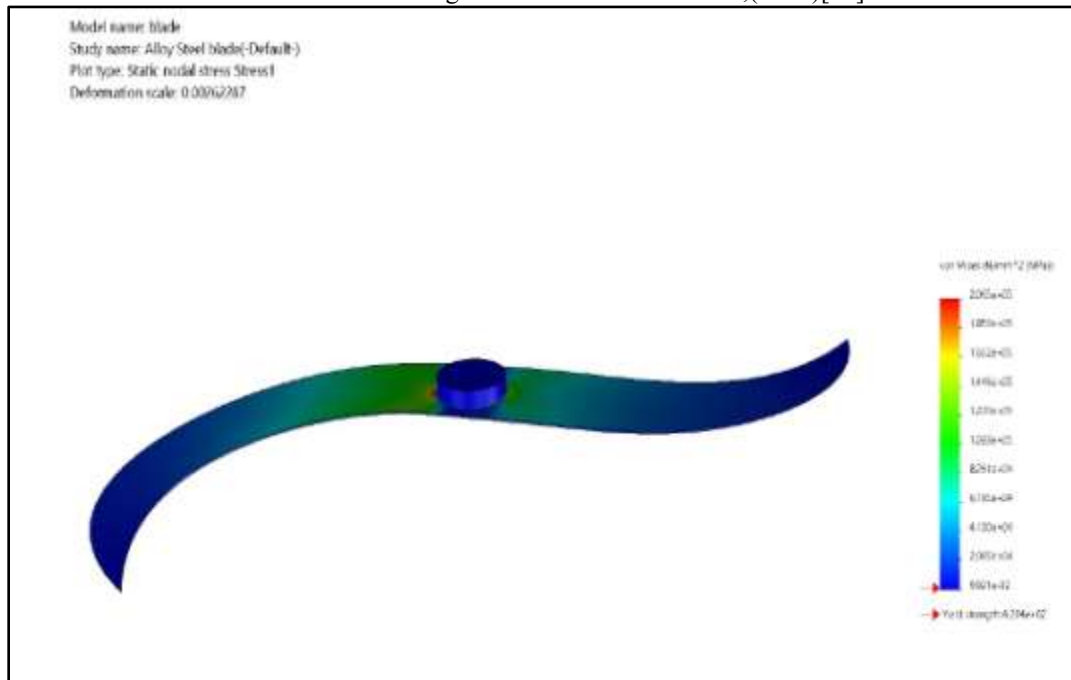
Fig. 6:- Static stress plot of alloy steel blade.
