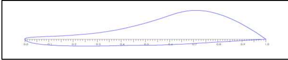
Fig.3:- NACA 5616 profile.
