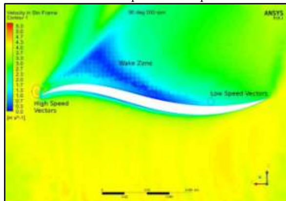
Fig. 7. (e):- Velocity Contour of blade at 90° with a rotational speed of 200 rpm.
