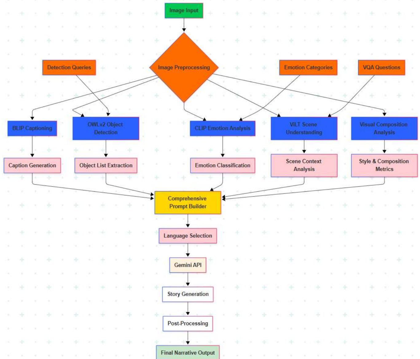
Figure 1:- A comprehensive diagram showing the integration of all AI models and data flow.
