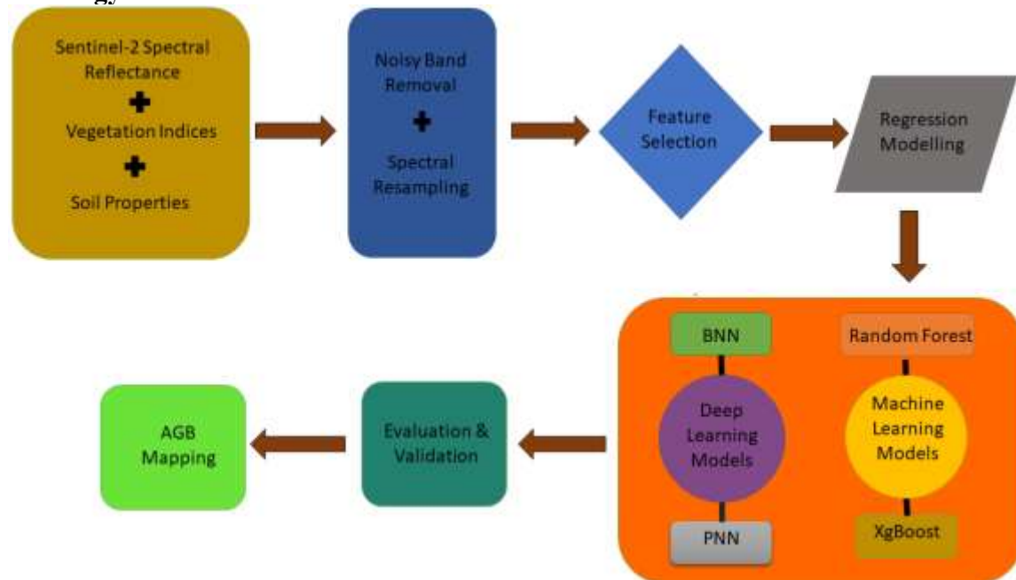
Figure 3:- Workflow for the AGB estimation modelling.
