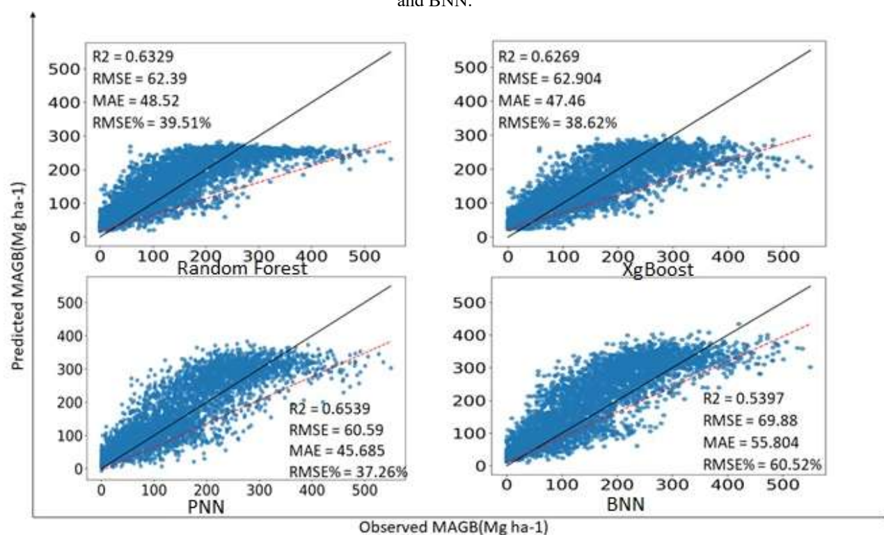
Figure 4:- Ypredictedvalues vs. Y plot of AGB (excluding soil properties data) for XGBoost, Random Forest, PNN, and BNN.
