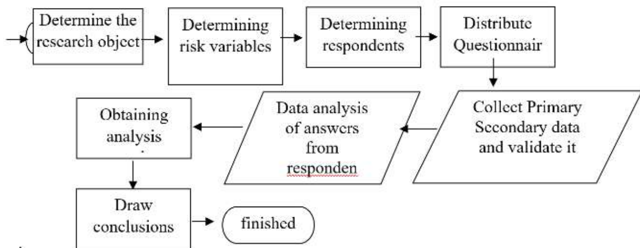
Fig.1:- Research Flowchart.
