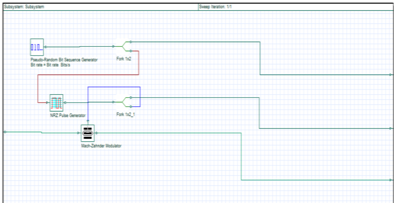
Figure 2:- Transmitter subsystem designed in Optisystem software.
