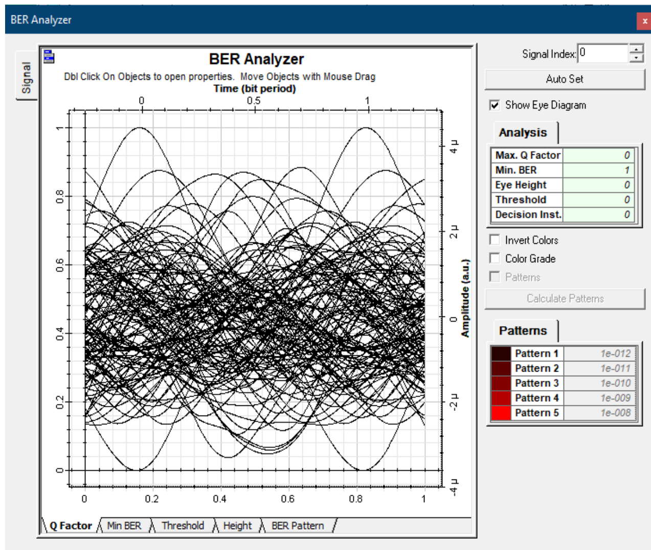
Figure 5:- Bit error analyzer output with only single mode optical fiber in transmission line.
