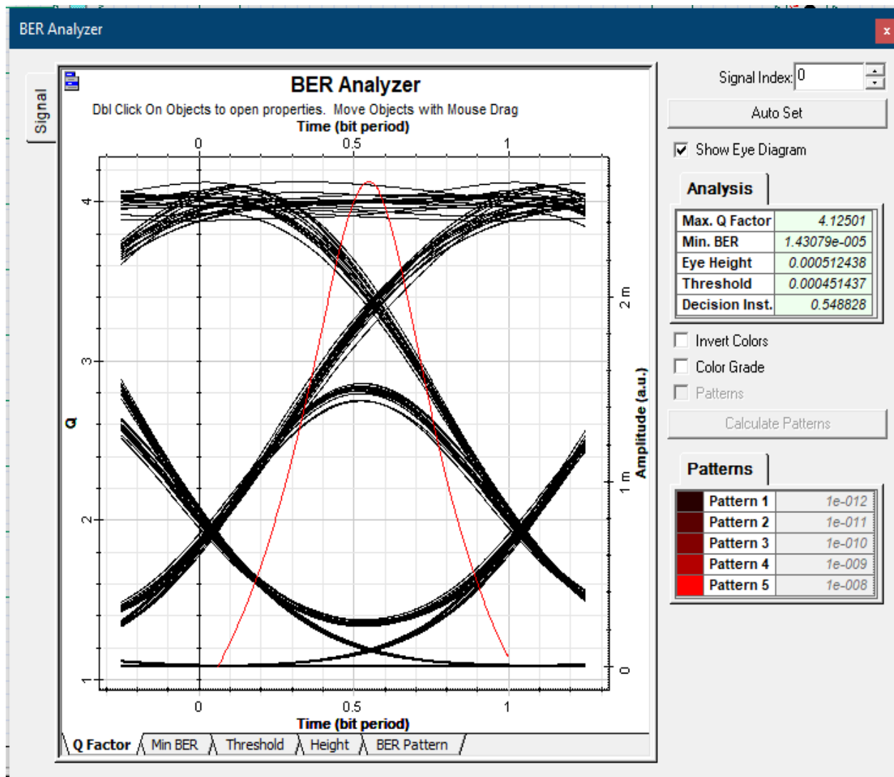
Figure 6:- Bit error rate analyzer output with SMF+EDFA+DCF as transmission line.
