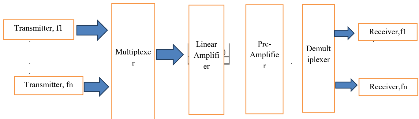
Figure 1:- Diagram of the DWDM communication system model.
