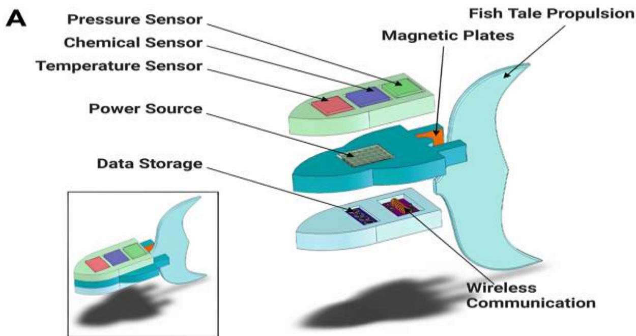
Figure 1:-Core structure of nanorobots with their components 3
