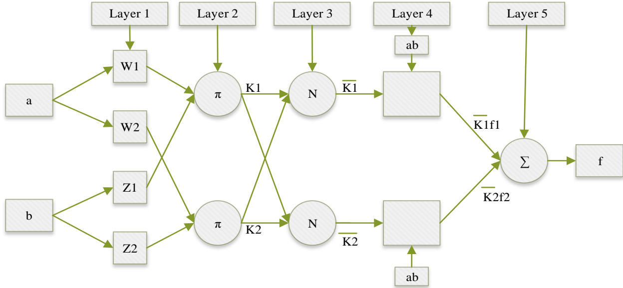
Figure 2:- General architecture of ANFIS.
