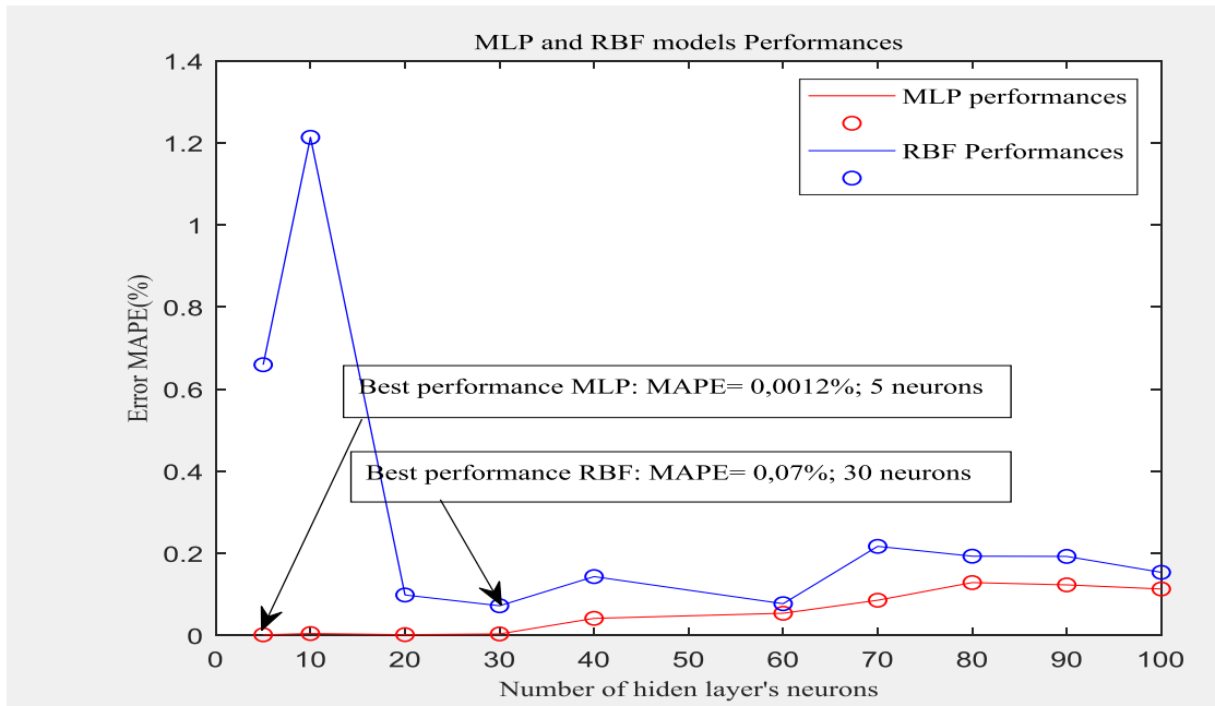
Figure 6:-MAPE error according to the number of hidden layer's neurons for MLP and RBF.
