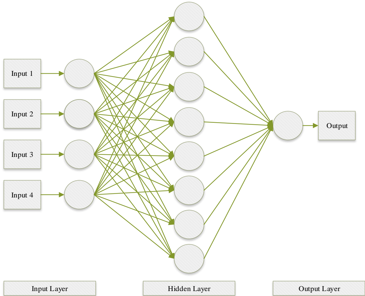
Figure 1:- Structure of two layers ANN.
